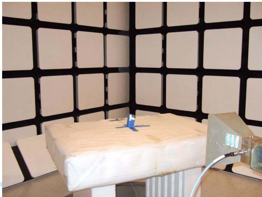
Test Configuration 2: 960 MHz to 40 GHz
