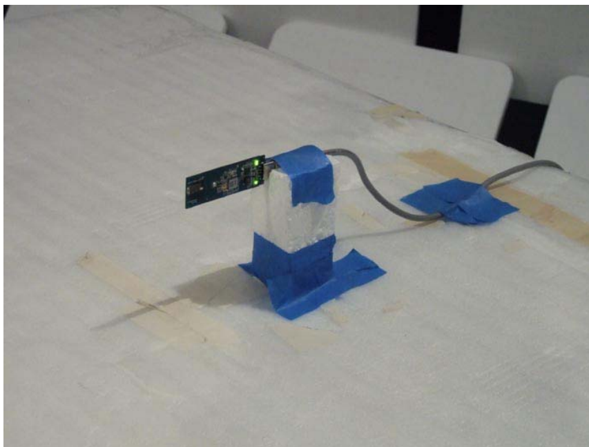
Worse Case EUT Setup [Vertical-orthogonal]:
