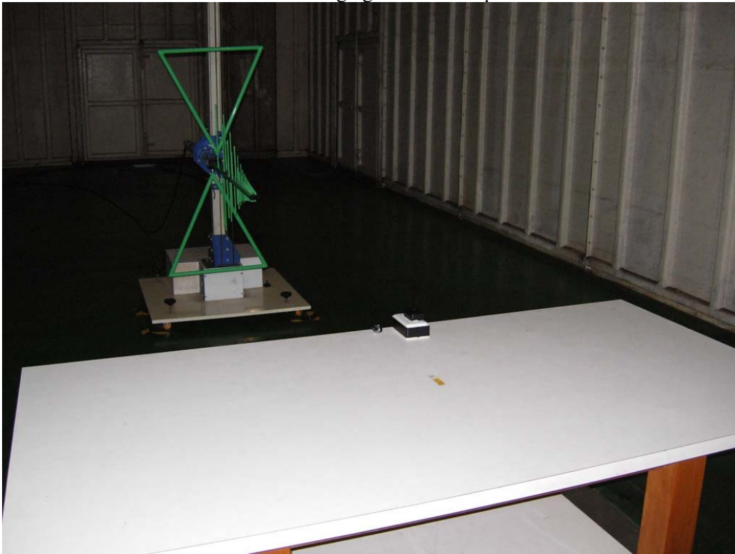
Back View of Radiated Test Mode 2: Charging with AC Adapter
