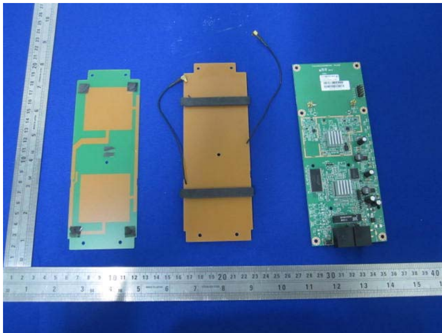
EUT – All Board Take Off View
