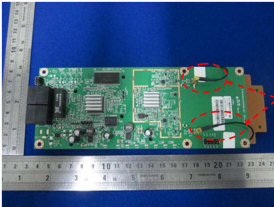
EUT –All Board Top View
