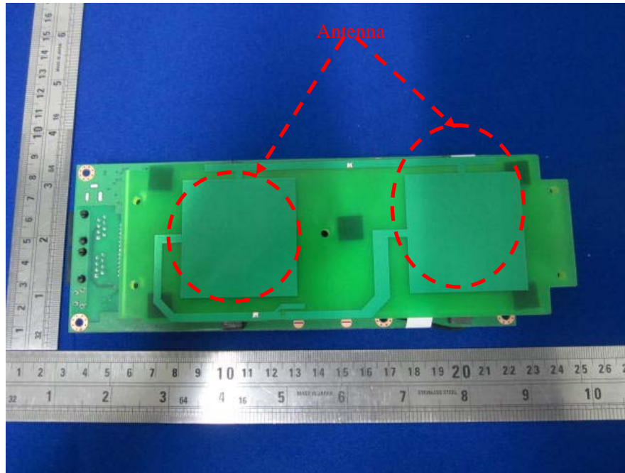
EUT –All Board Bottom View
