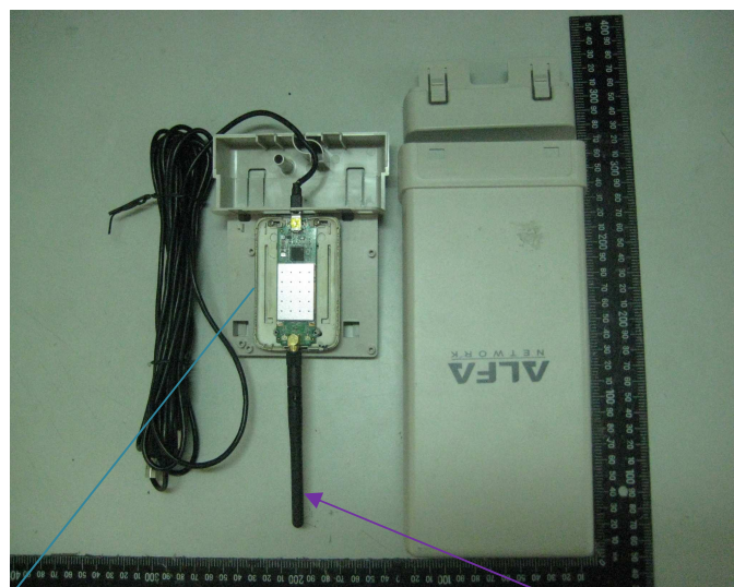
Inside View of EUT
