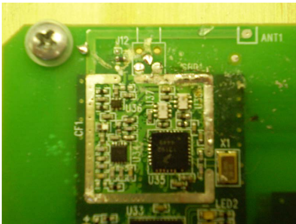
Close-up of RF Section, Shield Removed
