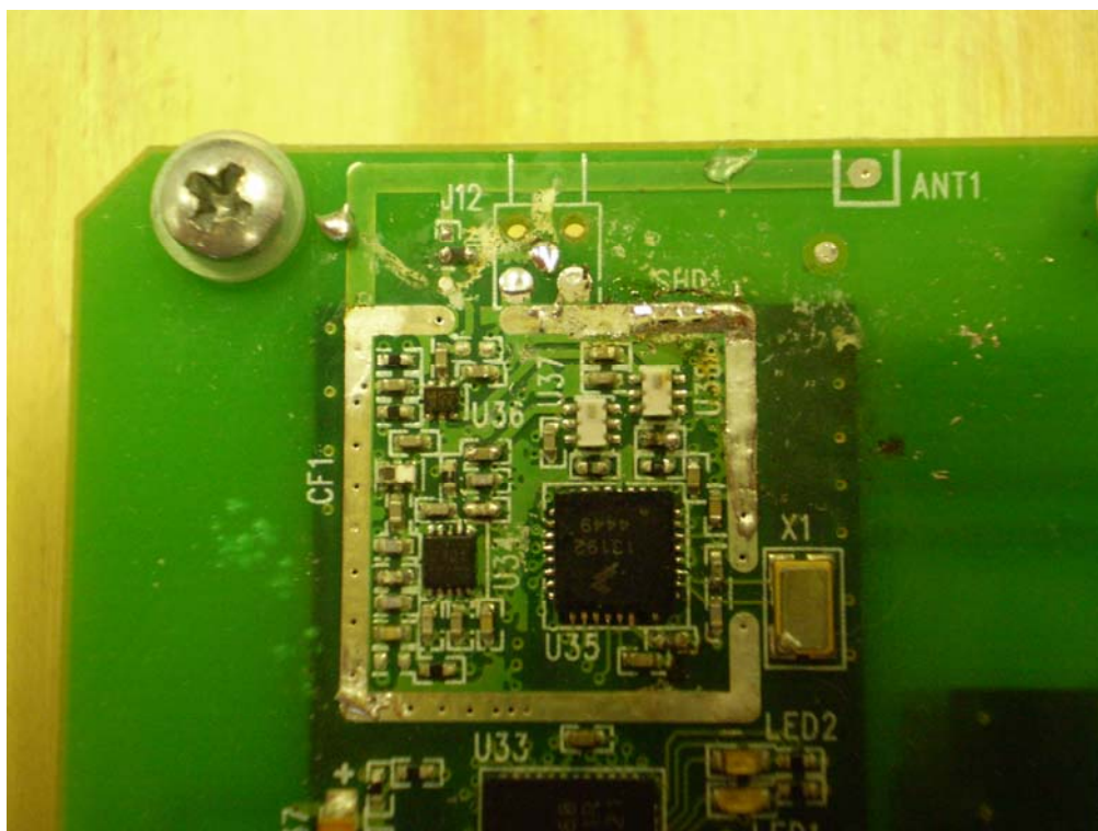
Additional View of RF Section, Shield Removed
