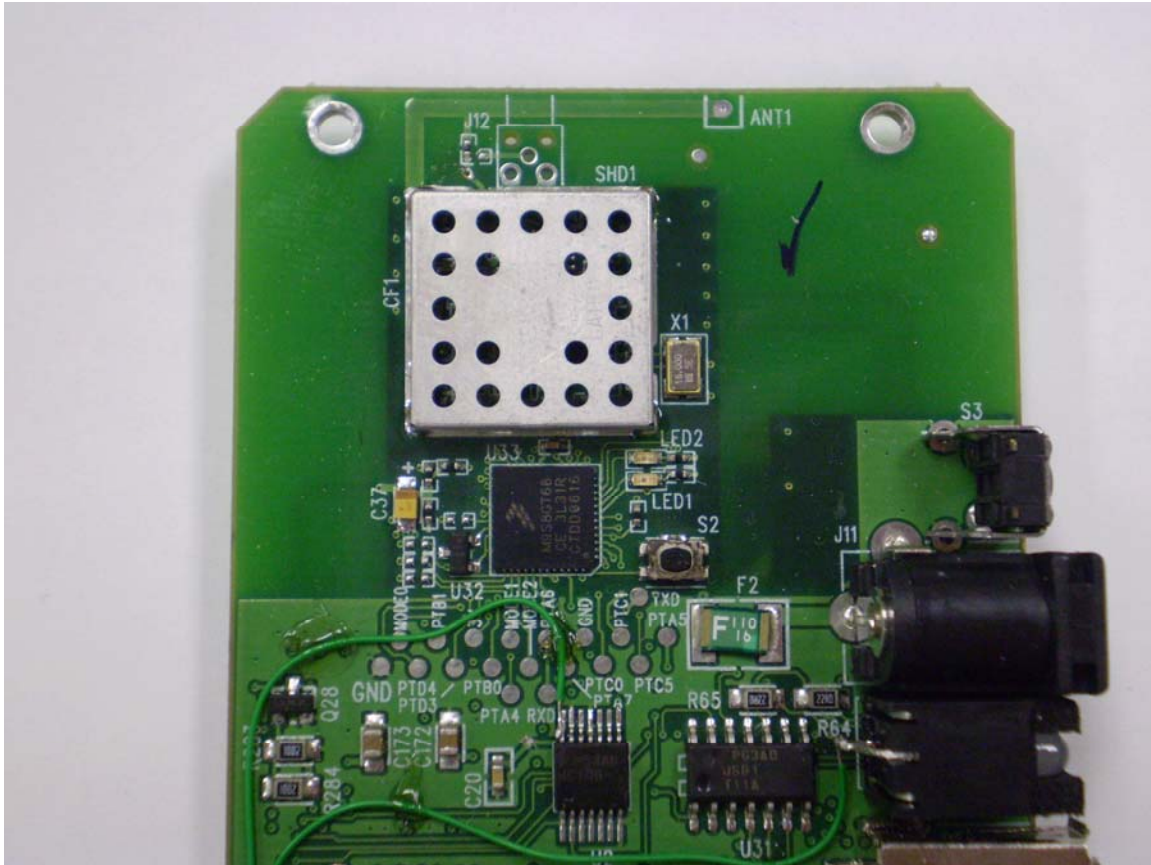
Close-up of RF Section, Shielded
