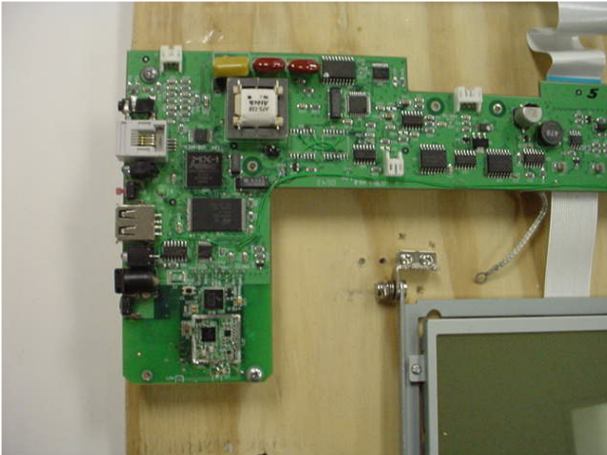
Photo Seven – Internal Close-up of RF Section, Left Side
