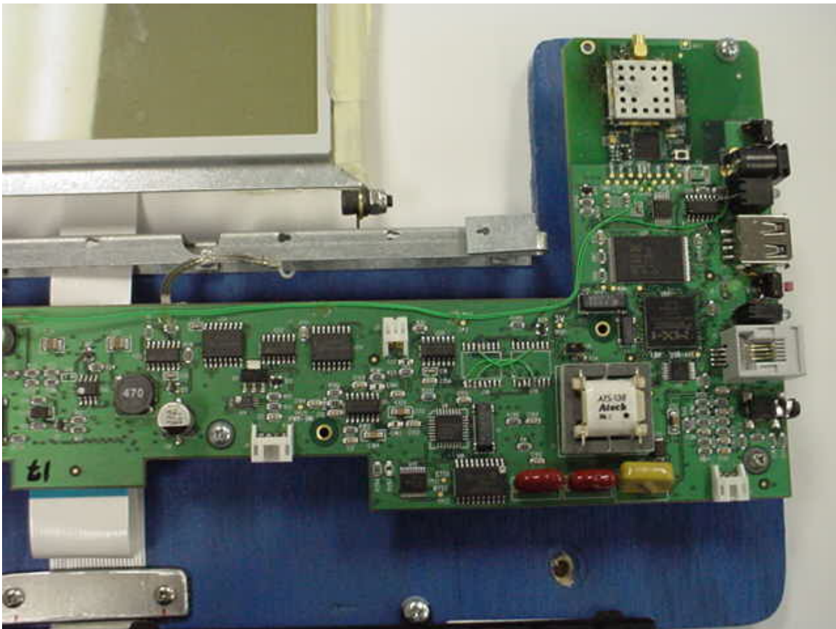
Photo Four – Internal Close-Up of RF Section, Right Side, Shielded
