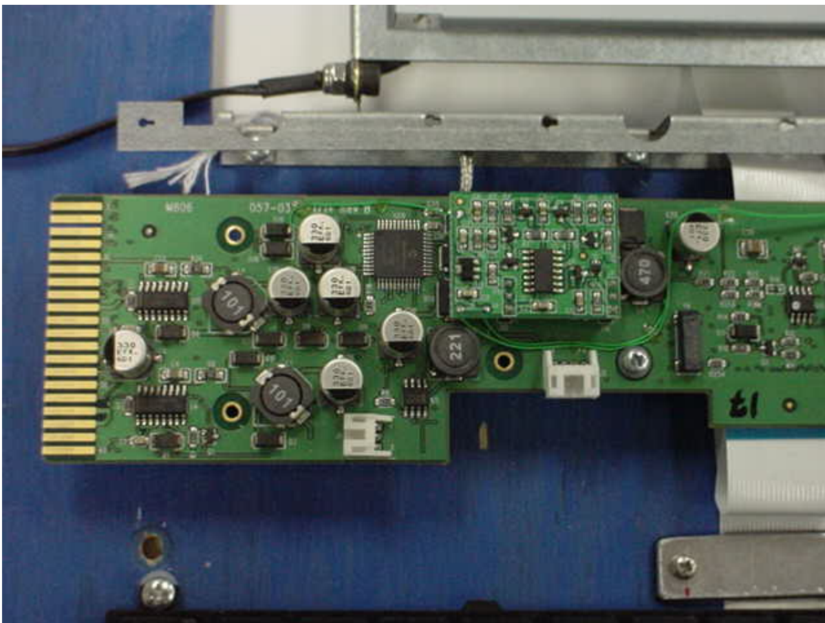
Photo Three – Internal Left Side of RF Section
