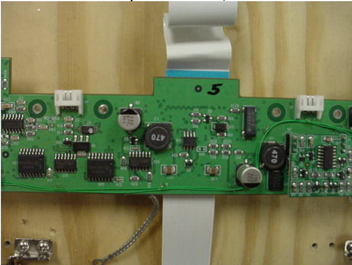
Photo Six – Internal Close-up of RF Section, Middle
