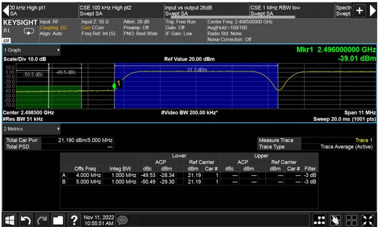
Plot of lower band edge for Low channels (2498.5 & 2503.5MHz)
