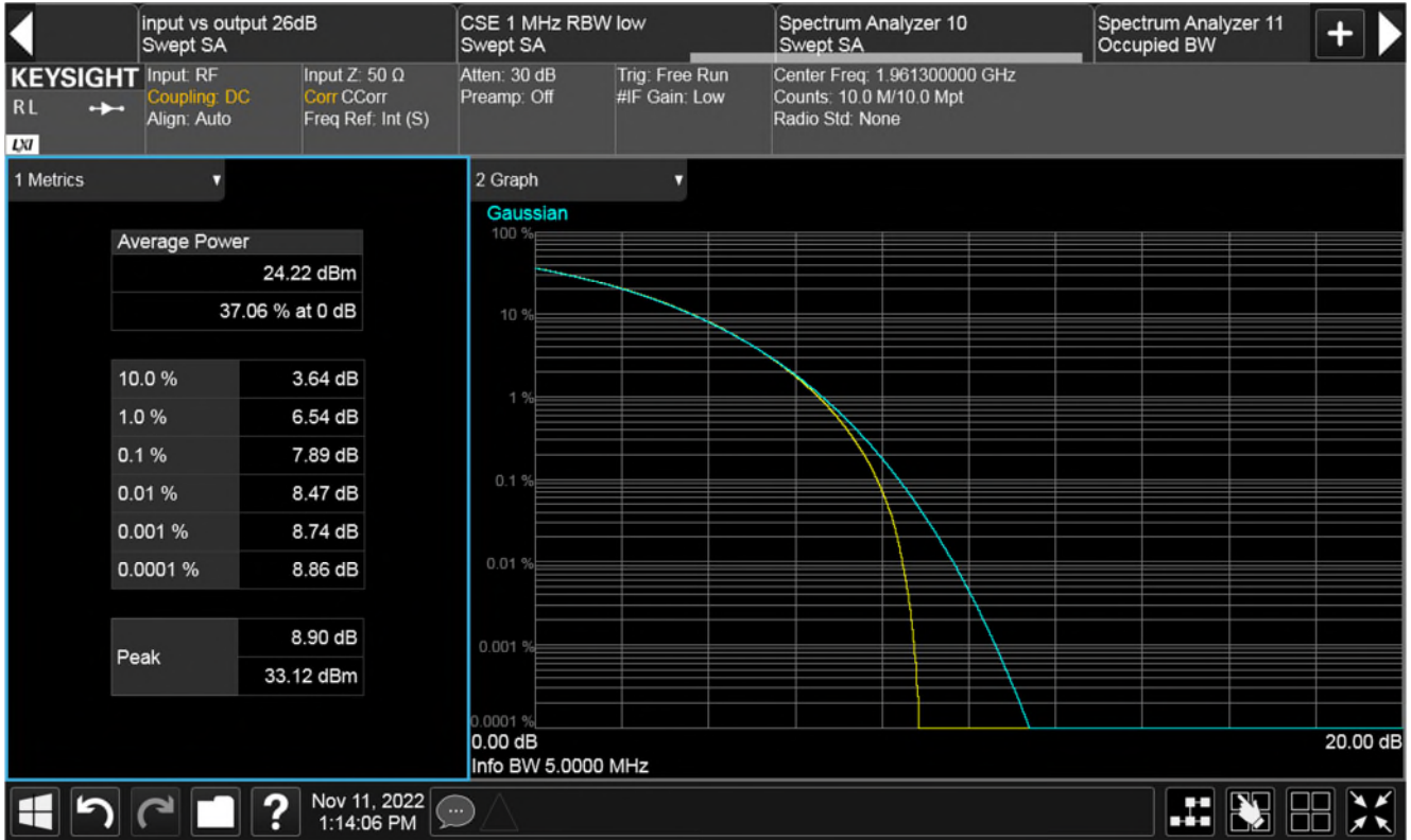
Plot of Peak to Average power ratio at determined f_0 in band 1930-1995 MHz (1961.3 MHz)
