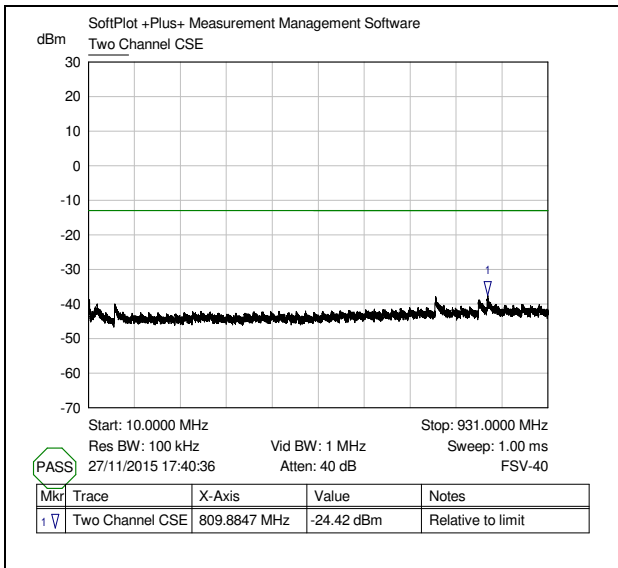
931 – 935MHz
