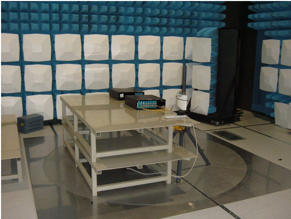
Hub and Remote Unit Test set-up
