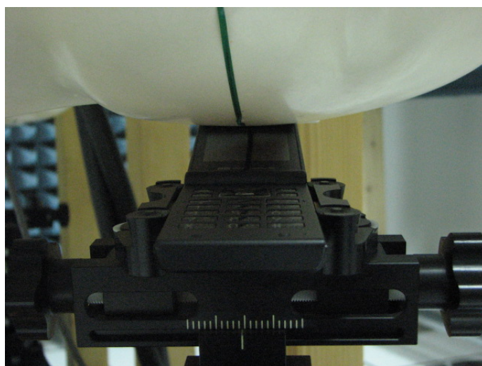
Fig 2 - Definition of the reference lines and points, on the phone and on the phantom and initial position
