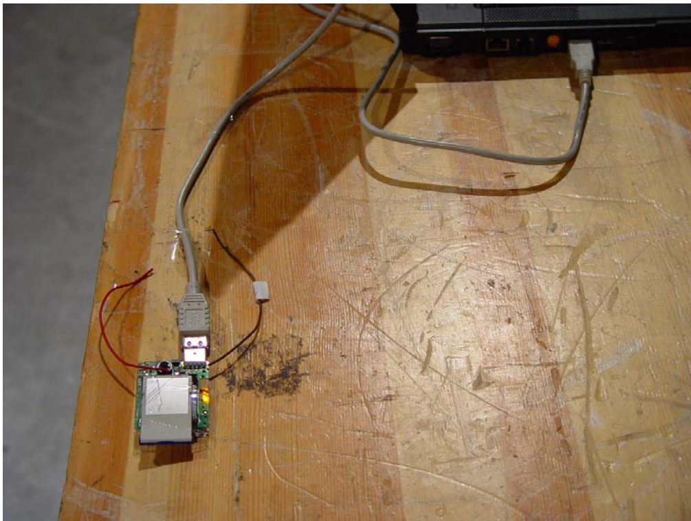
Radiated Emissions Test Setup 2
