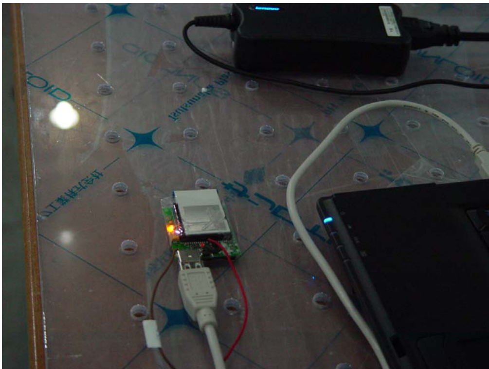
Conducted Emissions Test Setup 2
