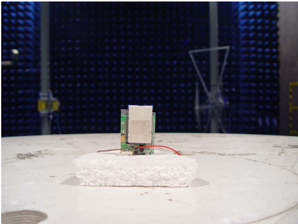
Radiated Spurious Emissions Test setup 2
