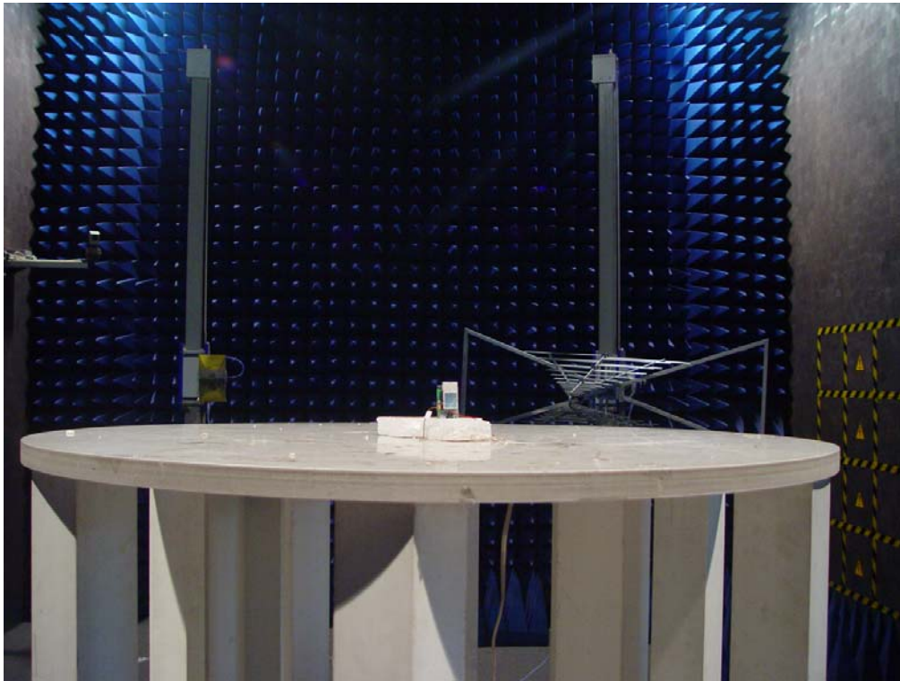
Radiated Spurious Emissions Test setup 1
