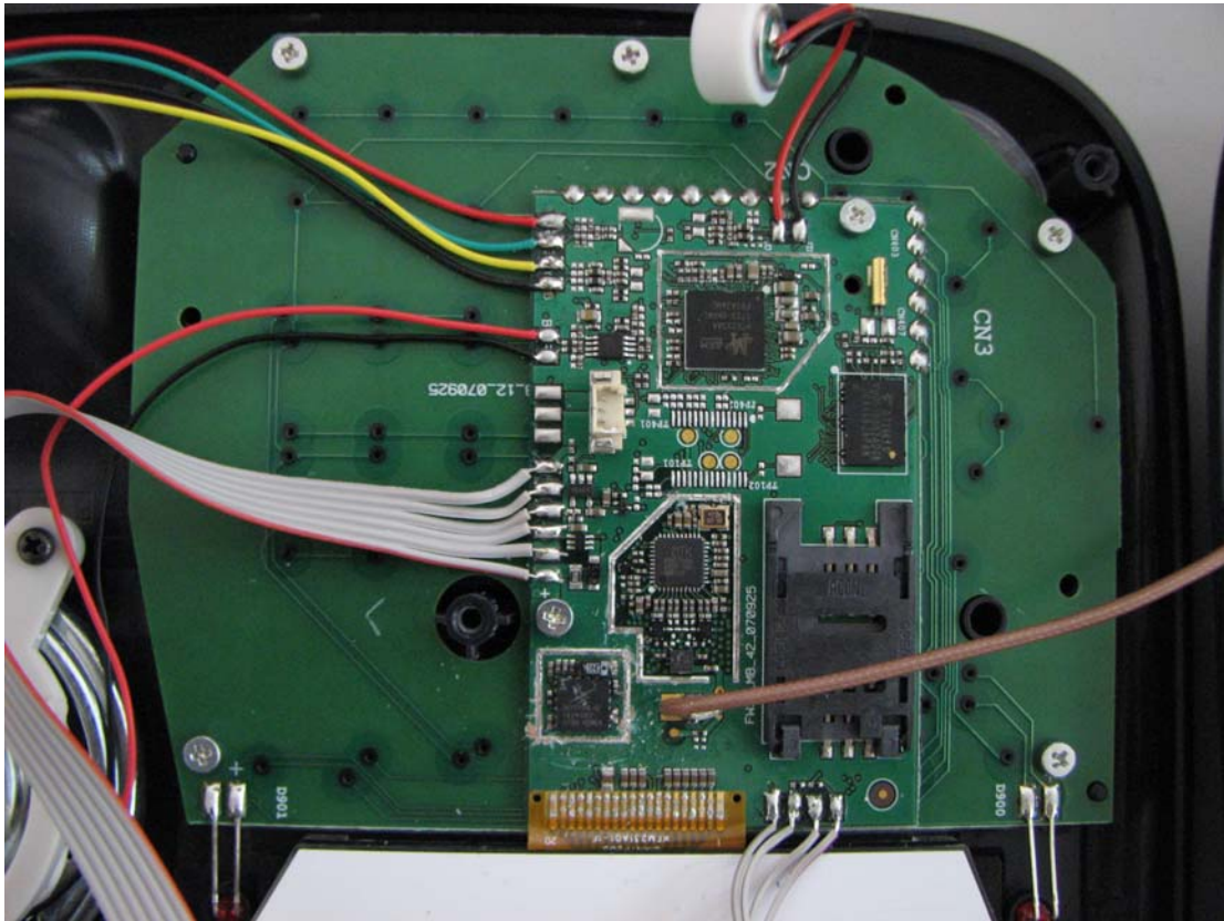
RF Module Board Top view
