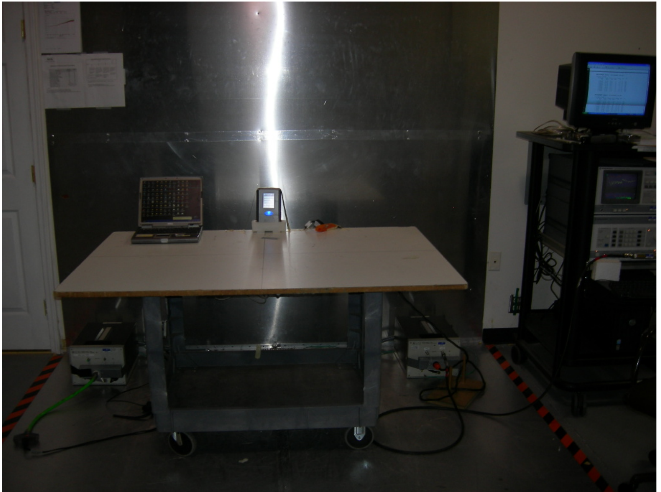
Figure 4: Conducted Emissions
