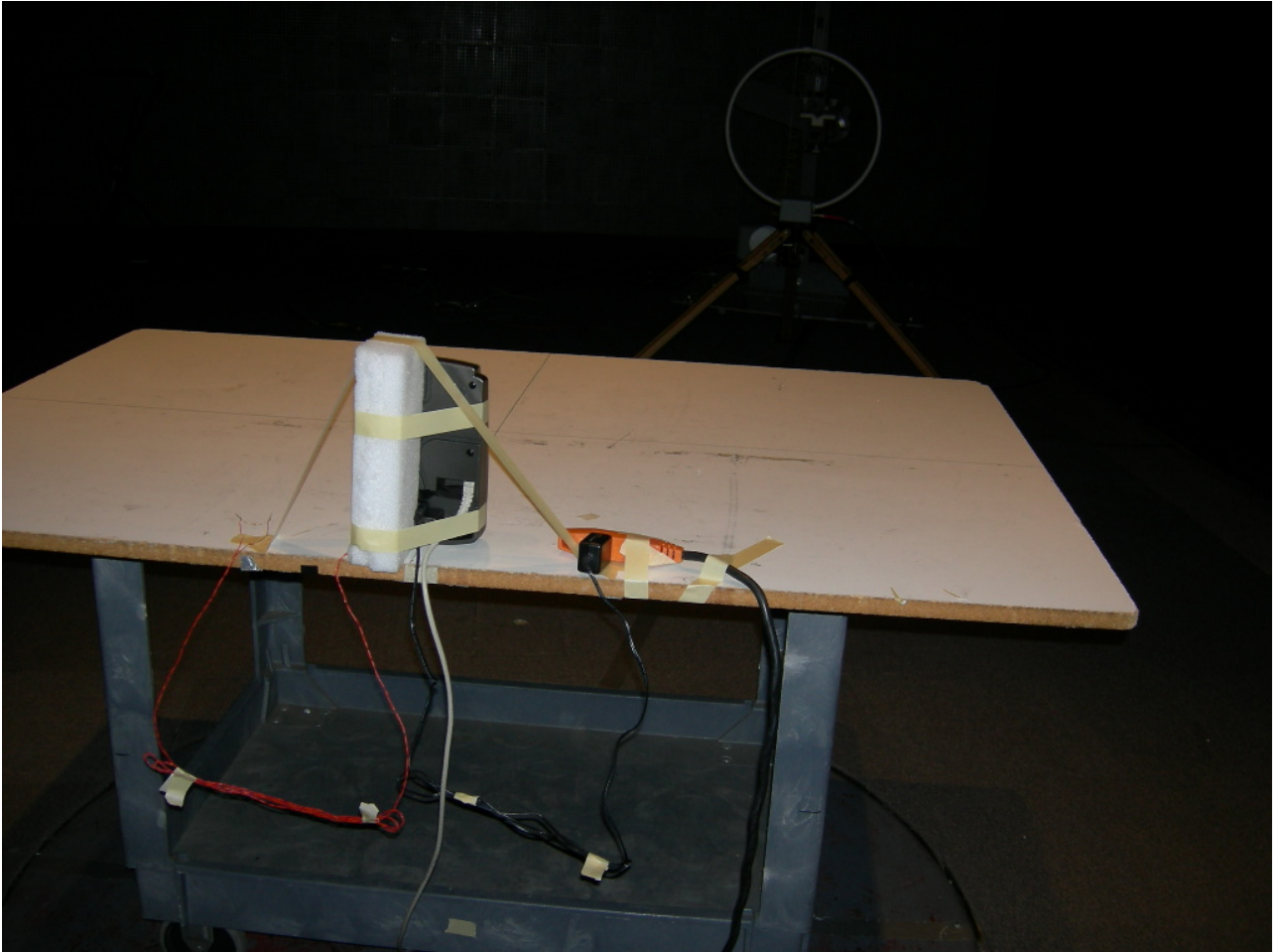
Figure 1: Intentional Radiated Emissions below 30 MHz
