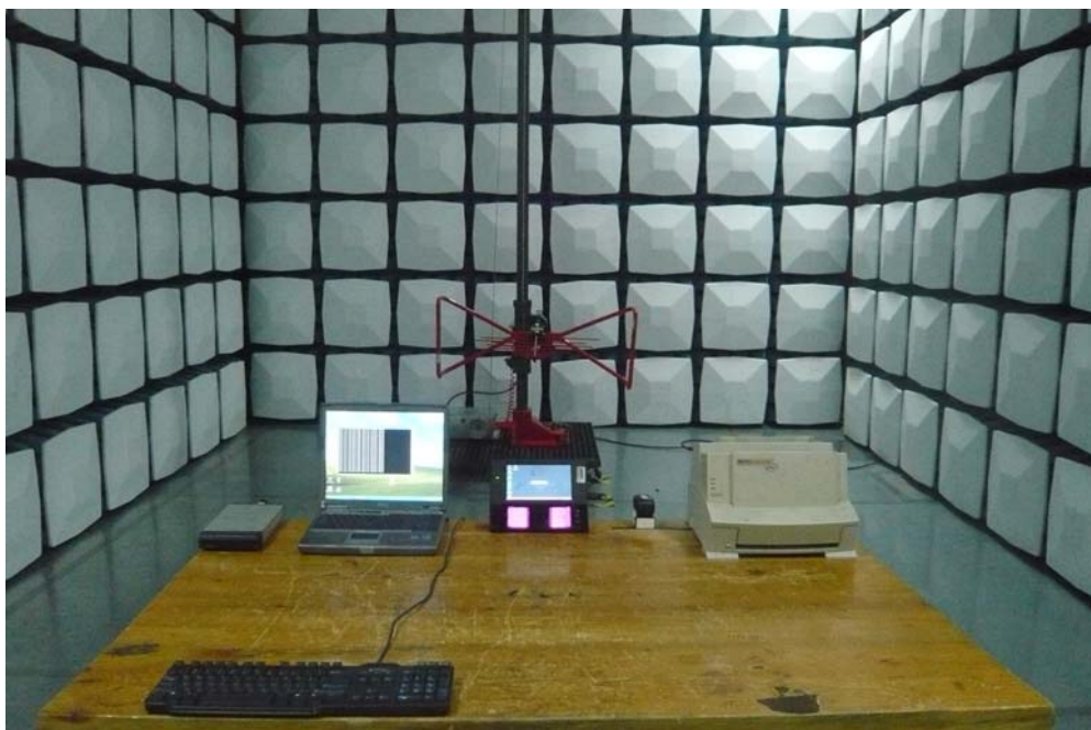
Radiated Emissions Below 1GHz - Front View
