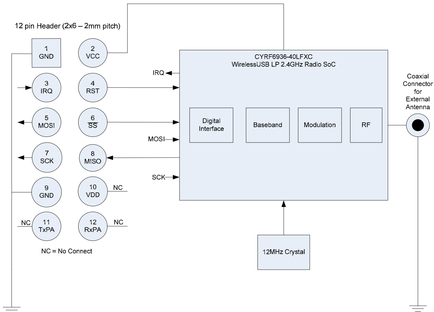
Figure 1 - Module Schematic
