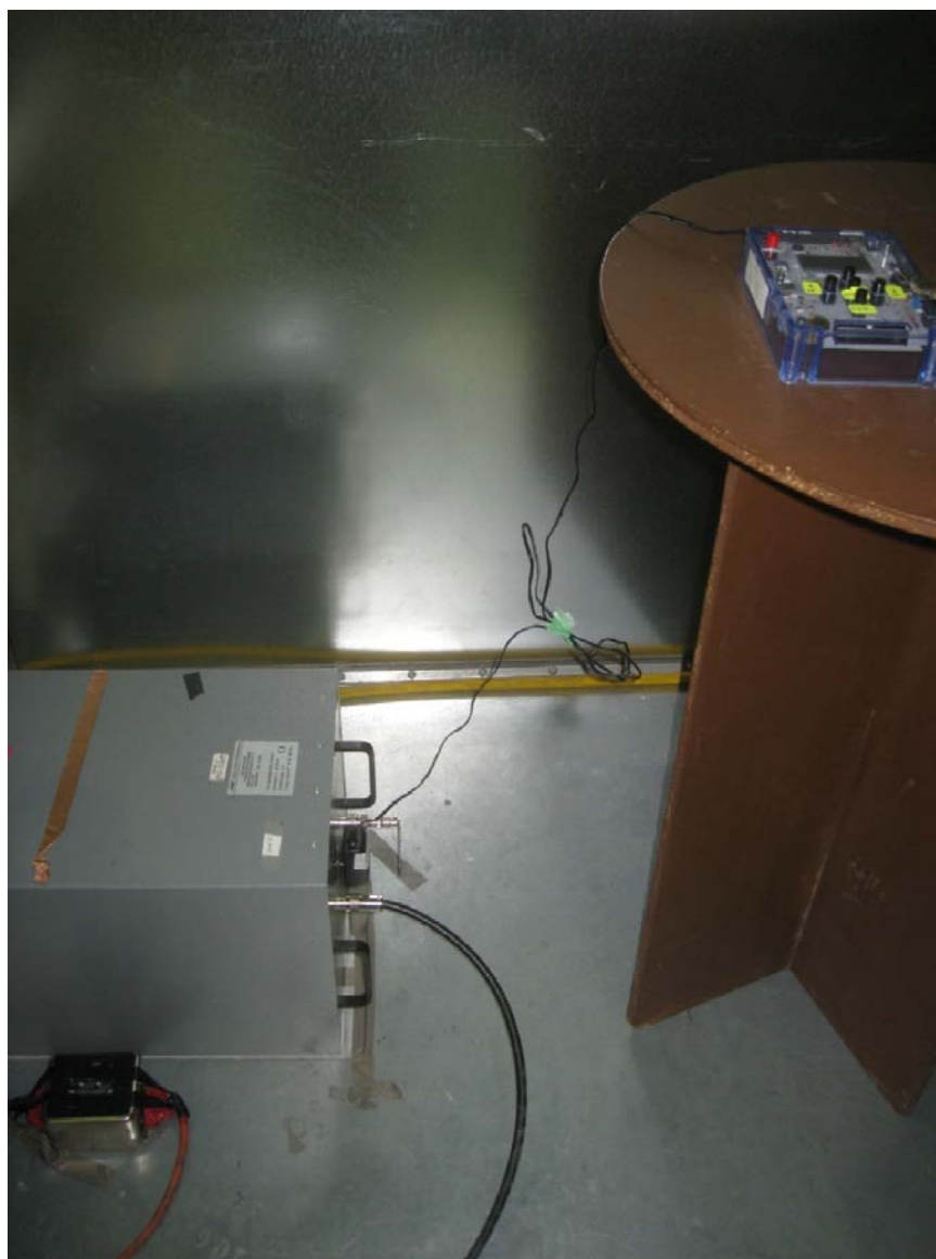
Power Line Conducted Emissions
