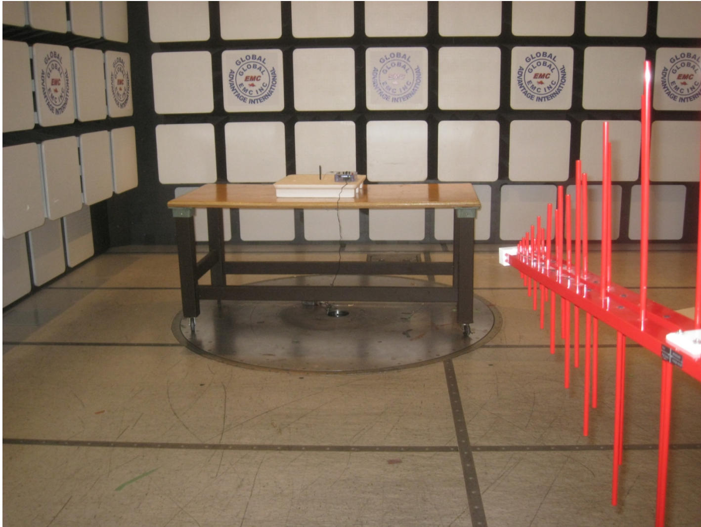
Radiated Emissions
