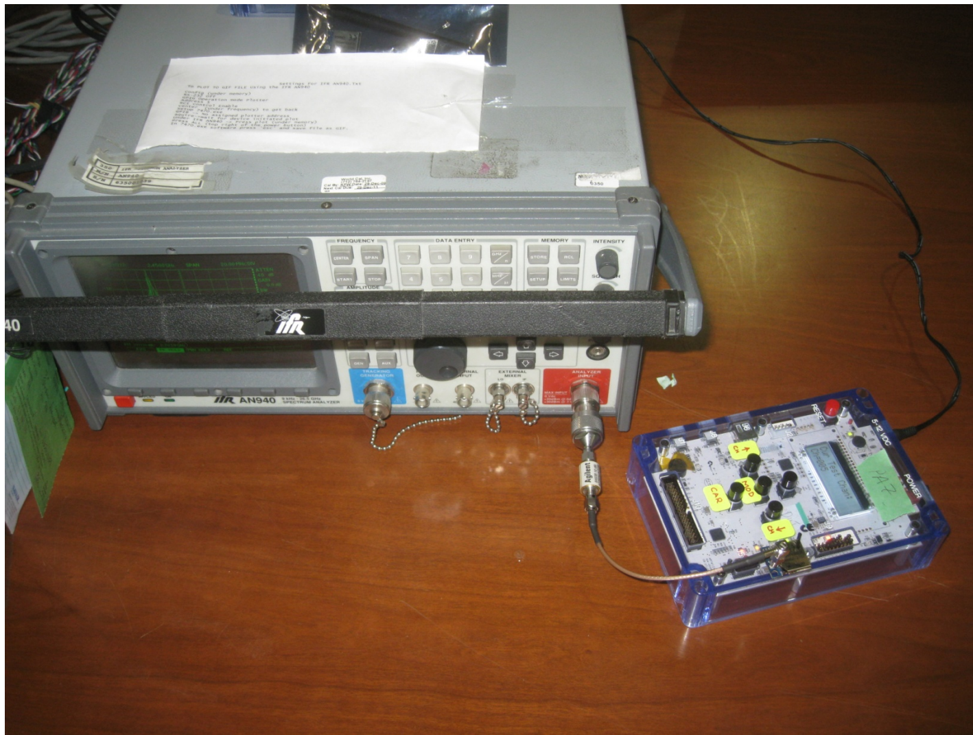
Antenna Conducted Emissions
