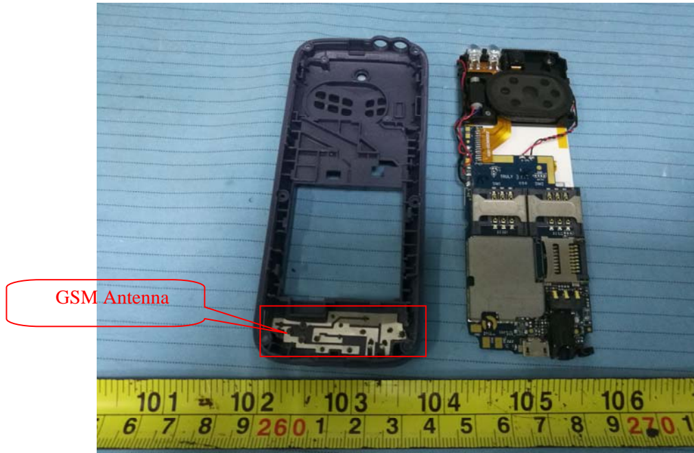
EUT – Cover off View 3
