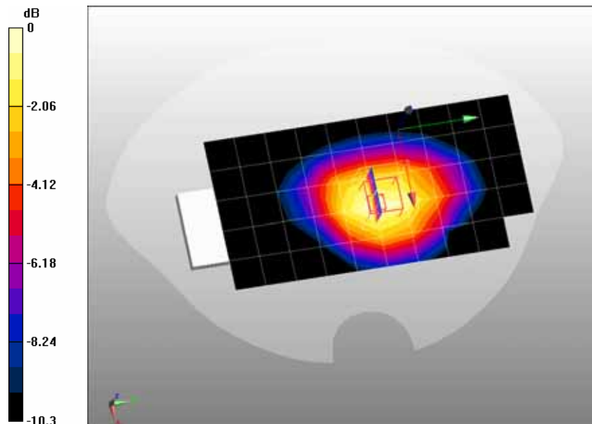
0 dB = 0.463mW/g
