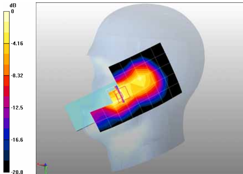
0 dB = 1.56mW/g
