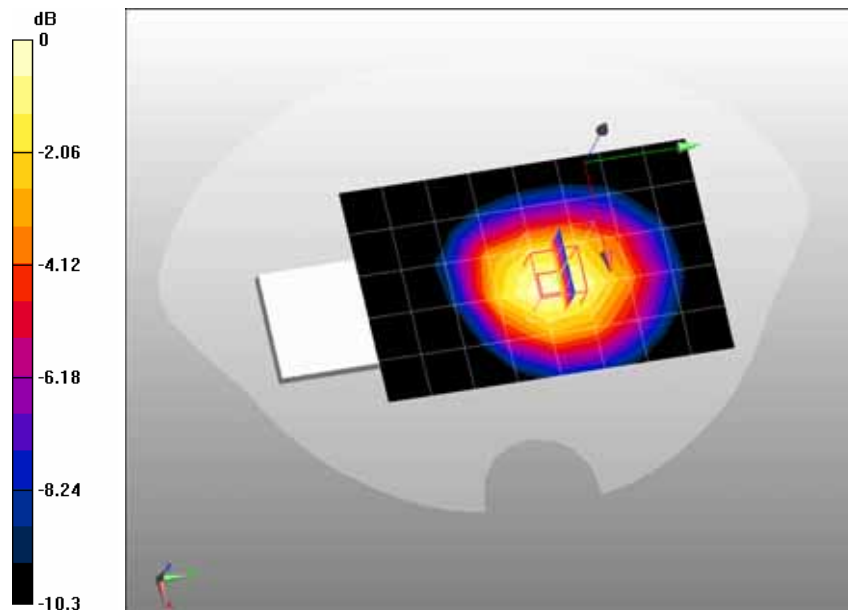
0 dB = 0.299mW/g
