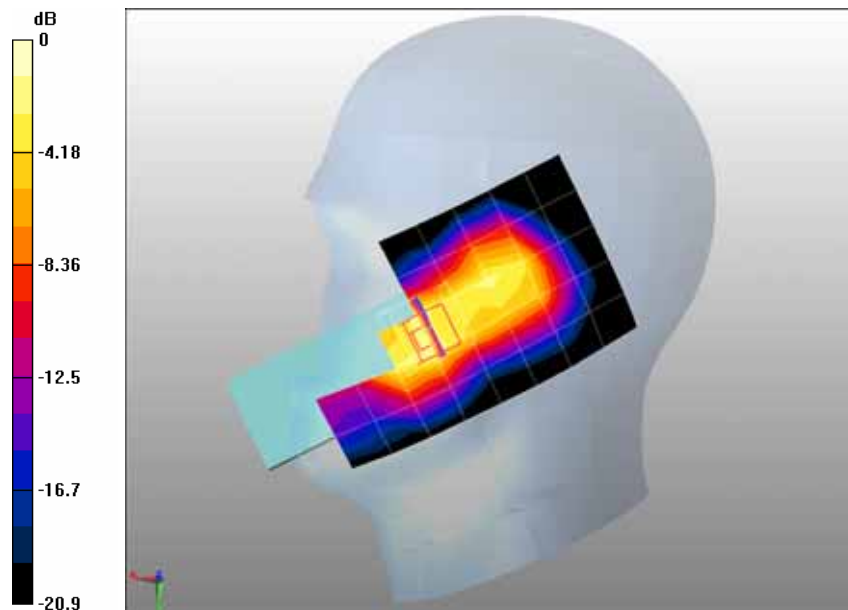
0 dB = 1.58mW/g
