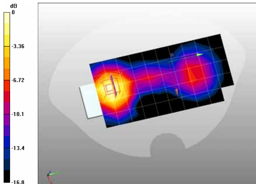
0 dB = 1.24mW/g
