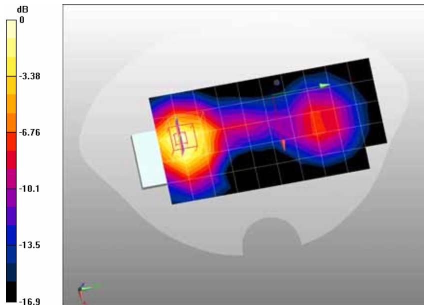
0 dB = 1.37mW/g
