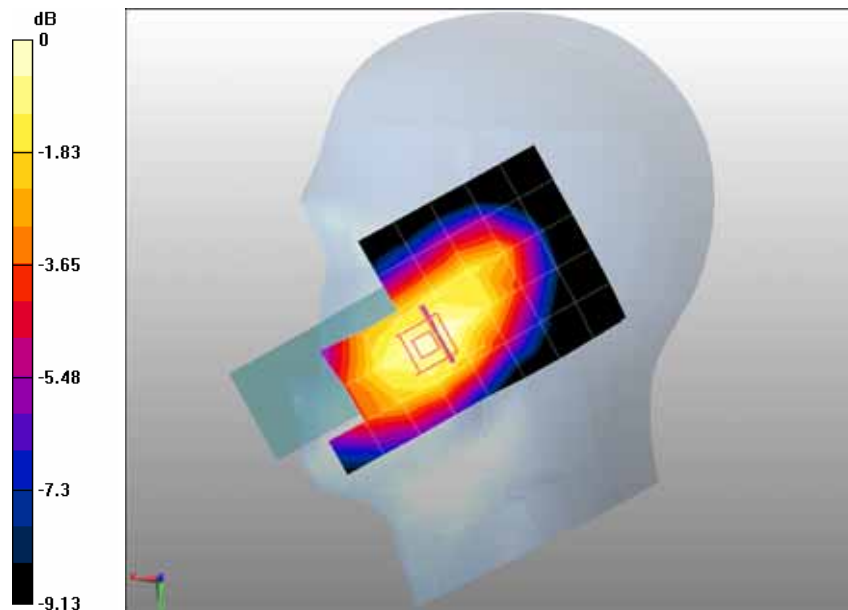
0 dB = 0.123mW/g
