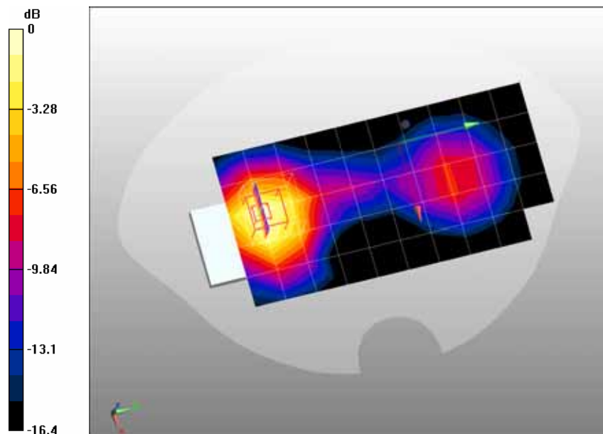
0 dB = 1.33mW/g
