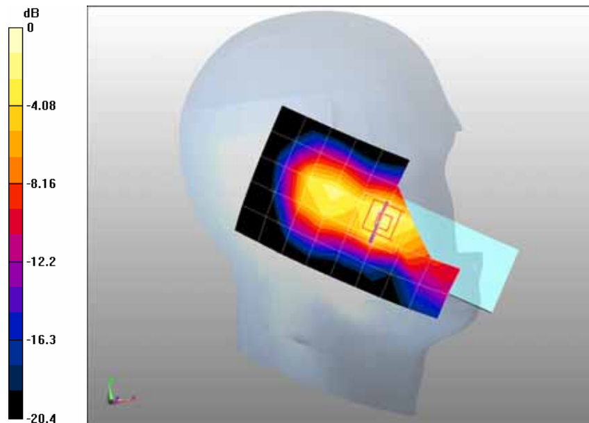
0 dB = 1.45mW/g
