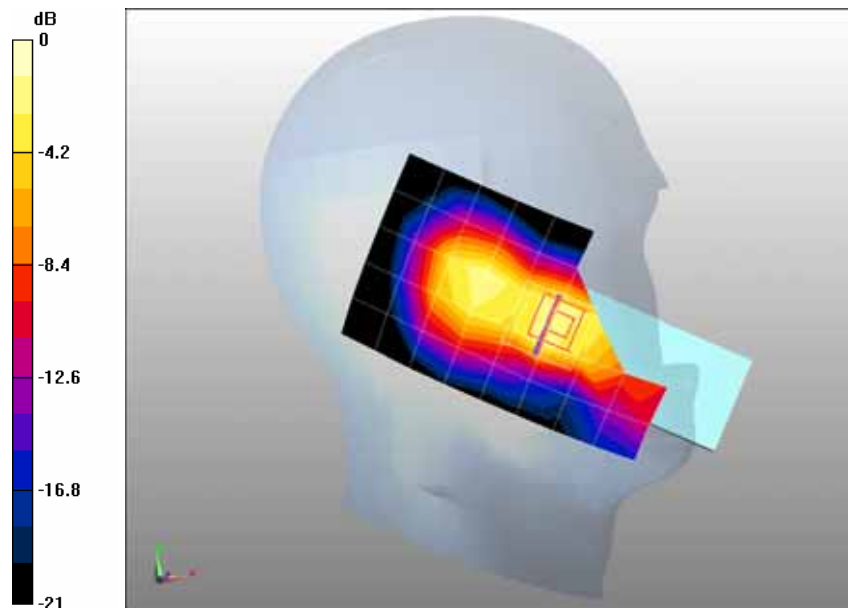
0 dB = 1.39mW/g
