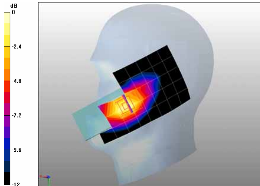
0 dB = 0.563mW/g
