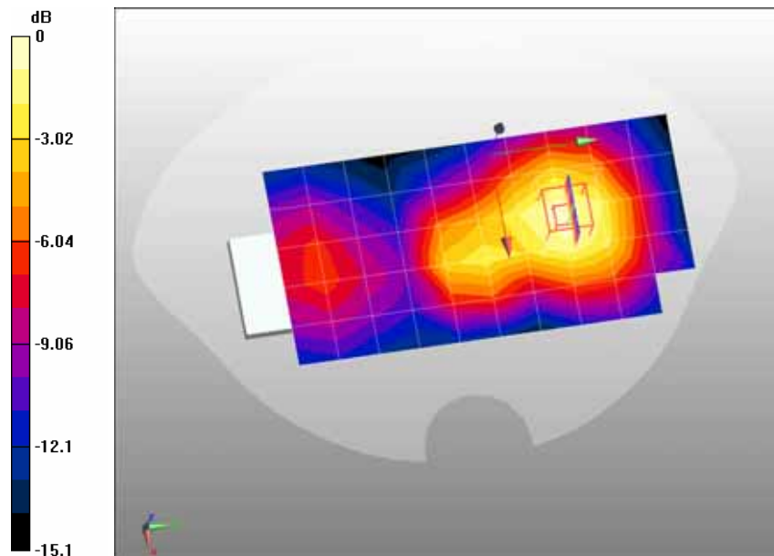
0 dB = 0.523mW/g
