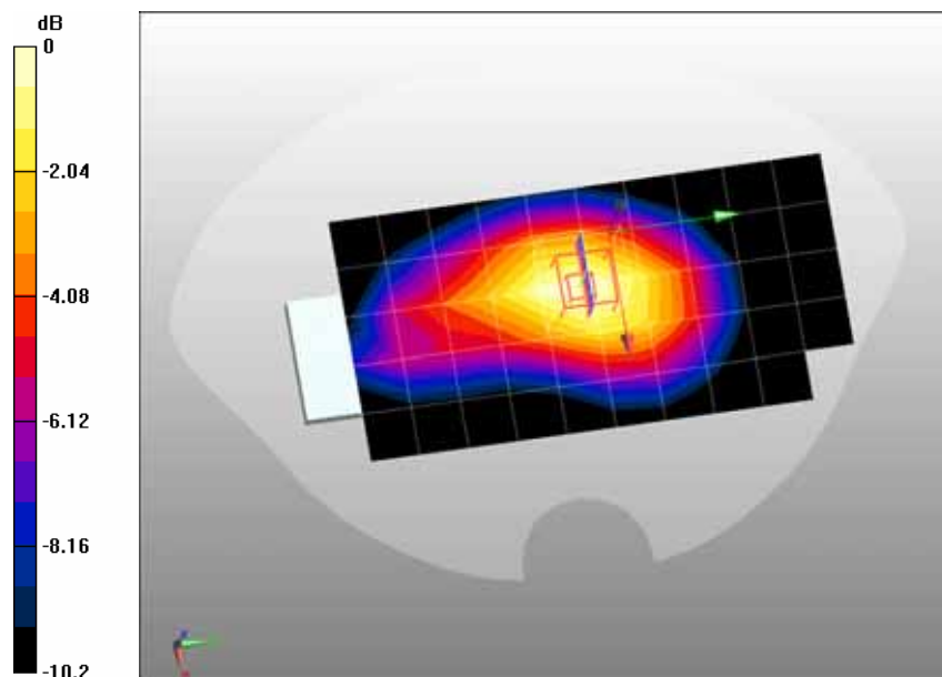
0 dB = 0.317mW/g
