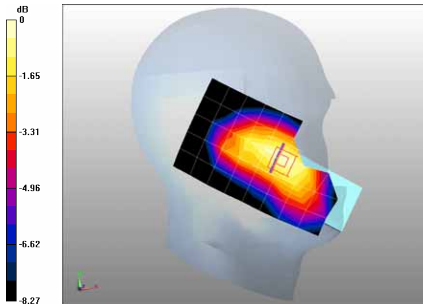
0 dB = 0.119mW/g
