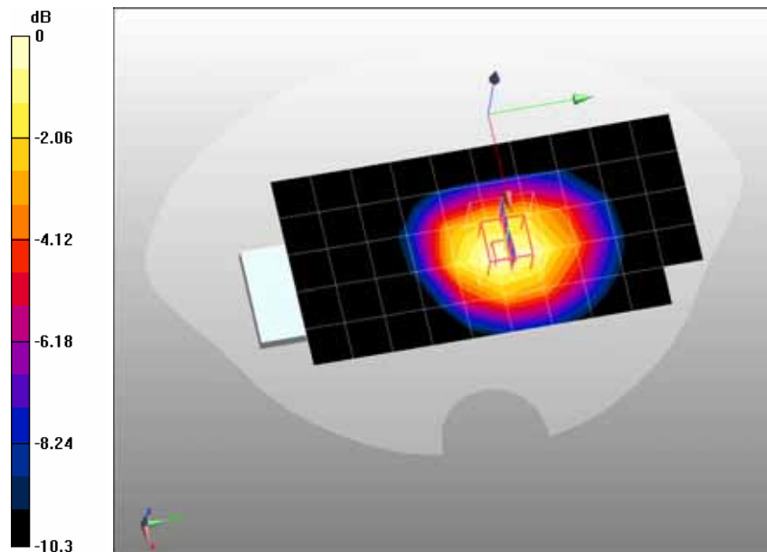
0 dB = 0.598mW/g
