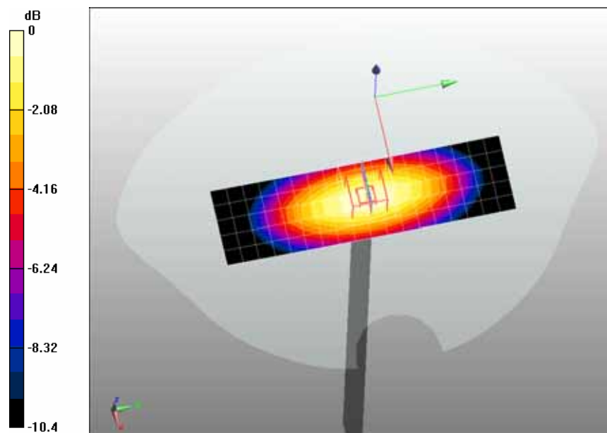
0 dB = 2.71mW/g
