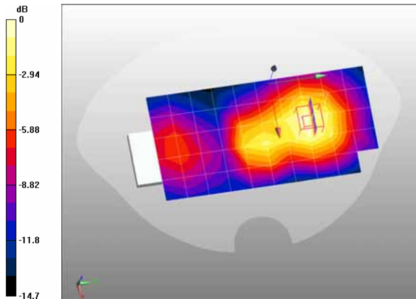
0 dB = 0.515mW/g
