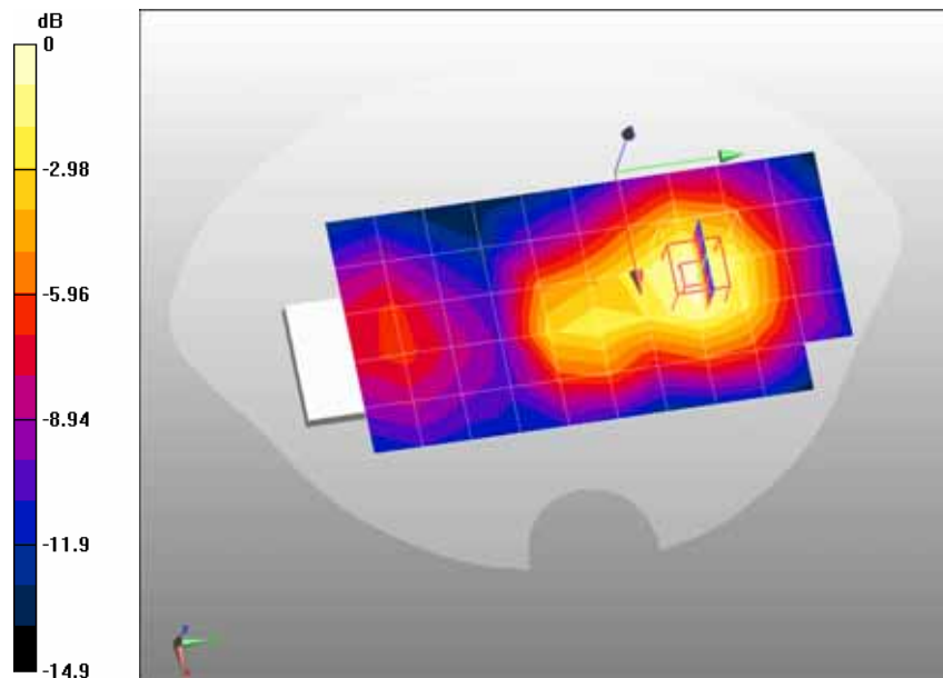
0 dB = 0.270mW/g
