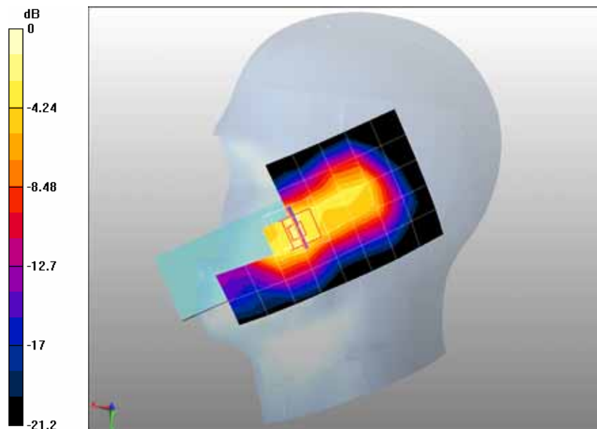
0 dB = 1.67mW/g
