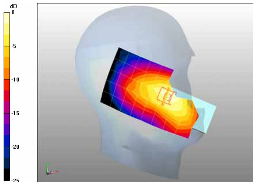
0 dB = 0.486mW/g
