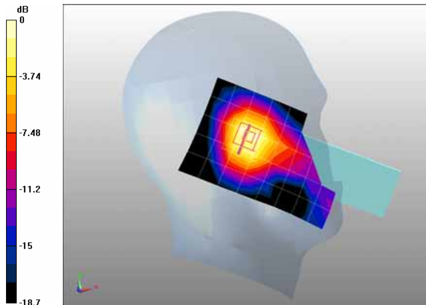
0 dB = 0.771mW/g
