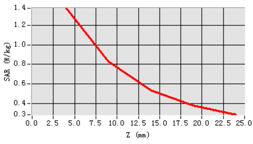
SAR, Z Axis Scan (X = -18, Y = -7)
