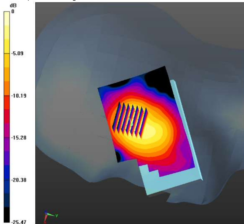
0 dB = 0.431 W/kg = -3.66 dBW/kg
