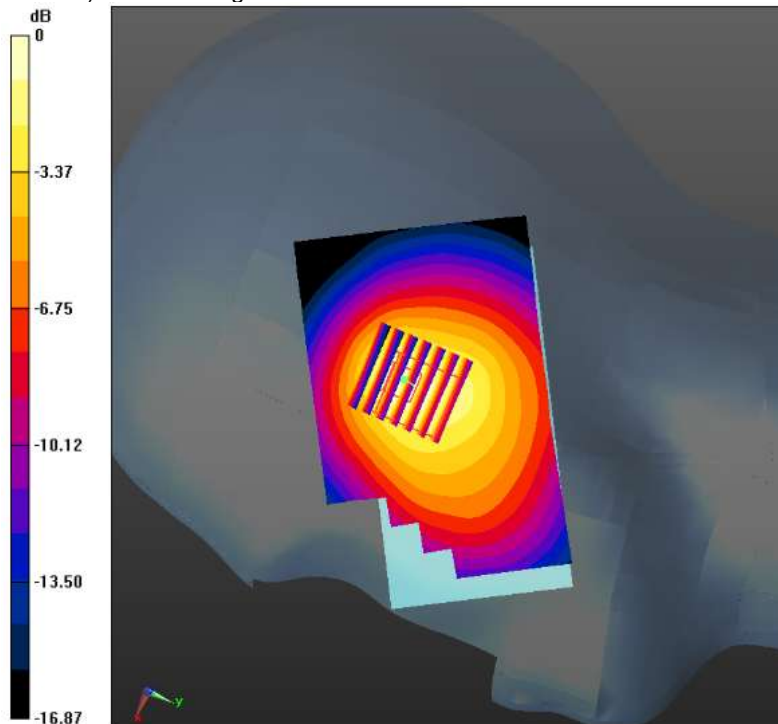
0 dB = 0.438 W/kg = -3.59 dBW/kg
