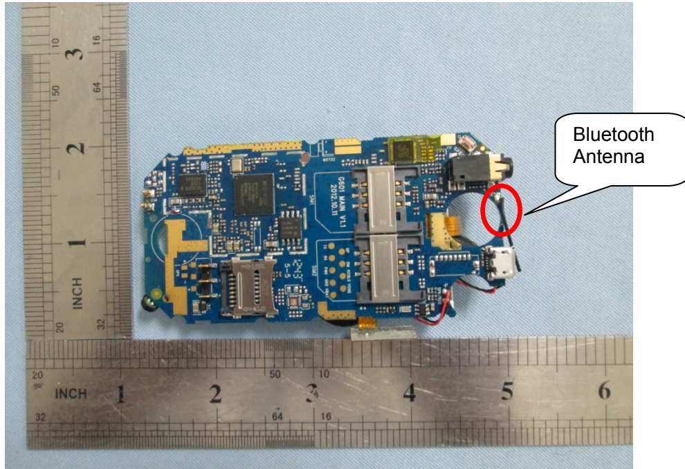
INTERNAL VIEW OF EUT-2
