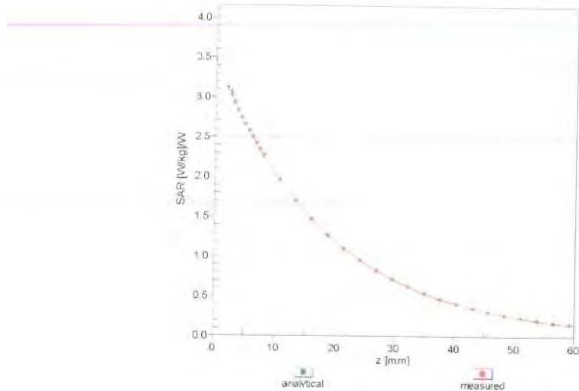
f = 835 MHz, WGLS R9 (H_convF)
