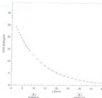
f = 1900 MHz, WGLS R22 (H_convF)
