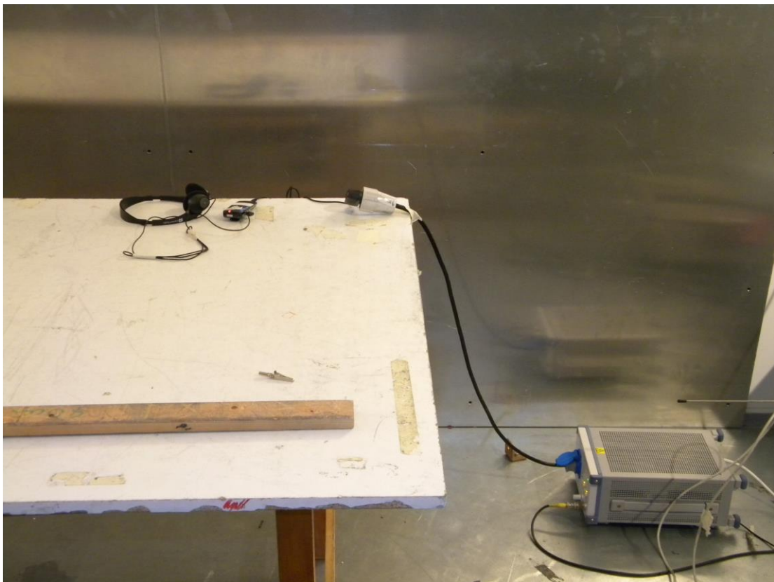
Photograph 2. AC power line conducted emissions test setup
