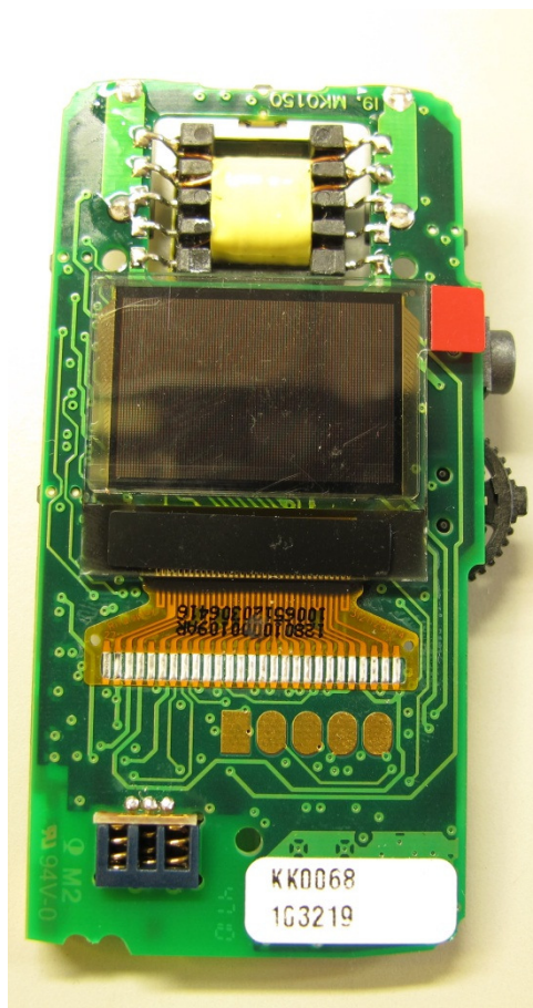
Rear enclosure part removed showing the PCB.
