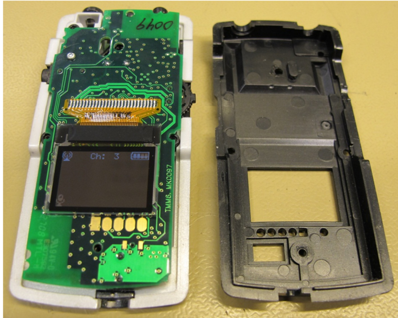
Rear enclosure part removed
