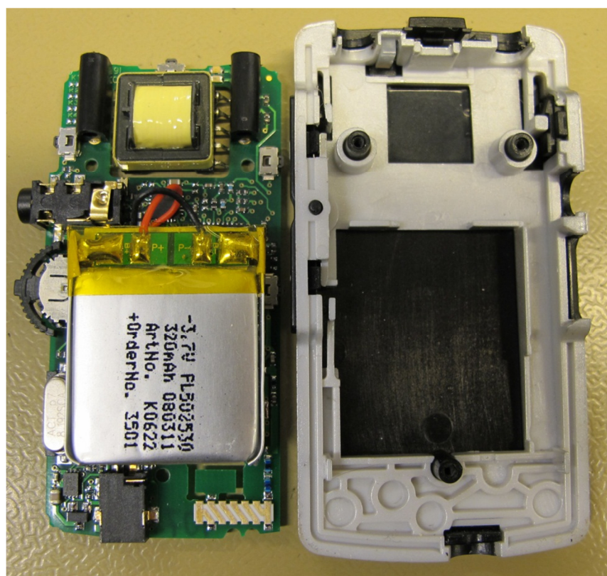
Top enclosure part removed
