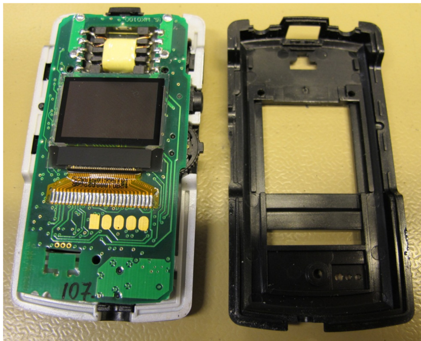
Rear enclosure part removed
