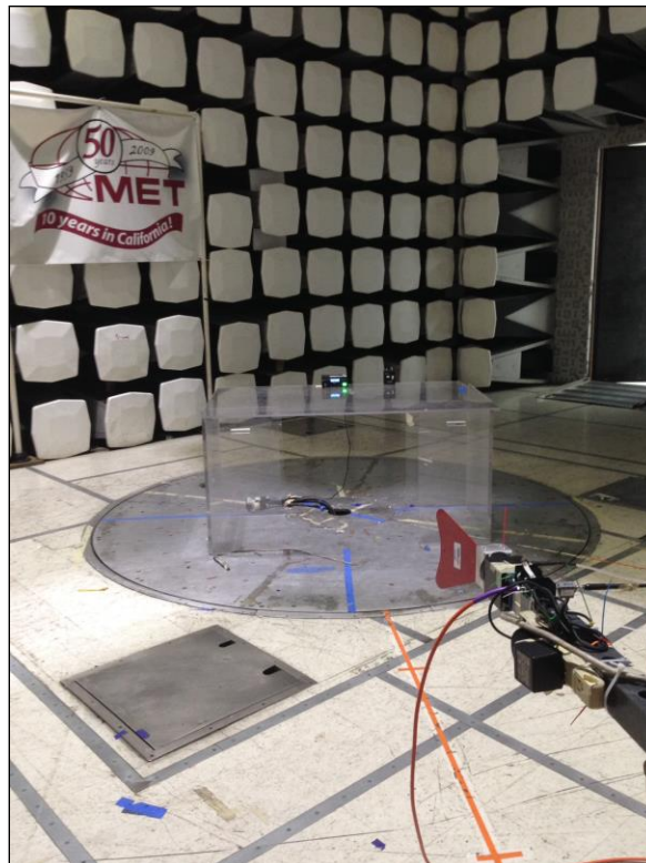
Photograph 2. Radiated Spurious Emissions, Test Setup, 2
