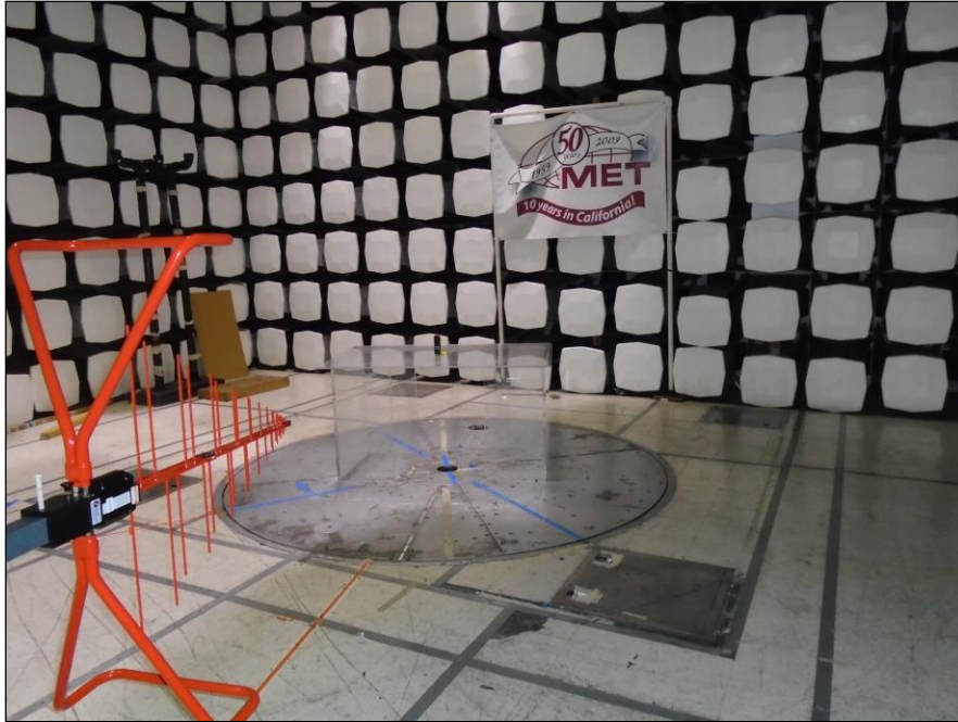
Photograph 1. Radiated Spurious Emissions, Test Setup, 1
