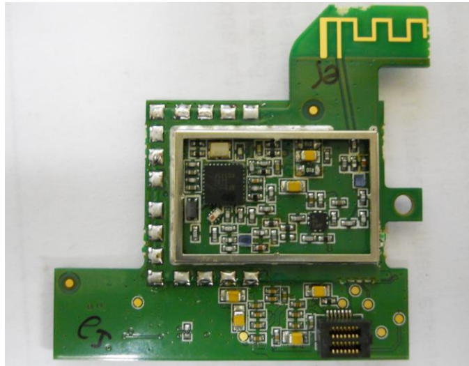
RF PCB
