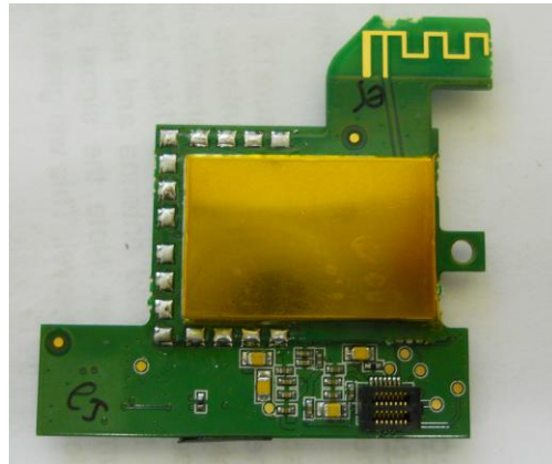
RF PCB
