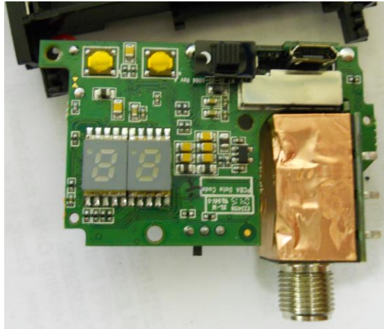
MAIN PCBA
