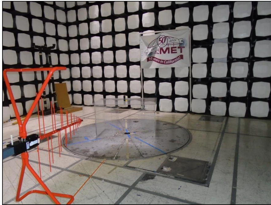
Photograph 2. Radiated Spurious Emissions, Test Setup, 1
