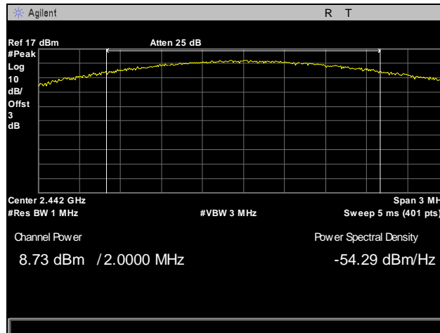
Plot 5. Peak Power Output, Mid Channel, Integrated
