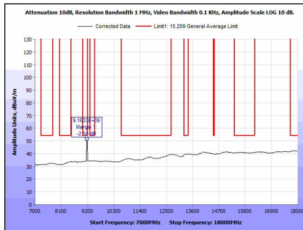
Plot 15. Radiated Spurious Emissions, Mid Channel, 7 GHz – 18 GHz, Average
