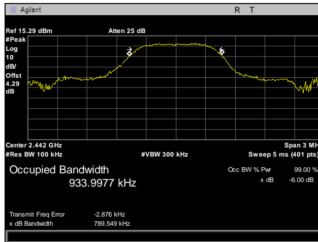
Plot 2. Occupied Bandwidth, Mid Channel
