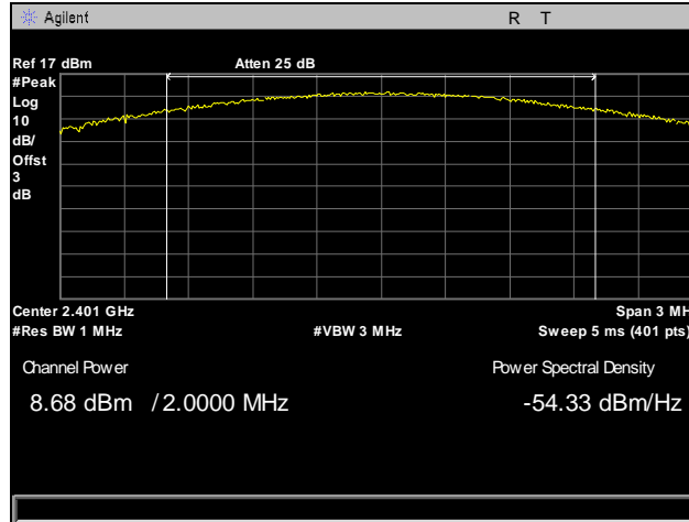
Plot 4. Peak Power Output, Low Channel, Integrated
