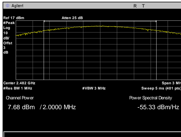
Plot 6. Peak Power Output, High Channel, Integrated
