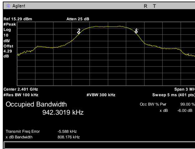
Plot 1. Occupied Bandwidth, Low Channel
