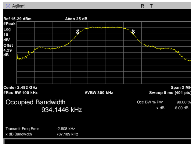
Plot 3. Occupied Bandwidth, High Channel
