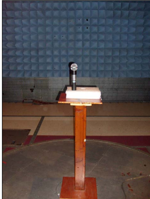
Photograph 4. Radiated Spurious Emission, Test Setup
