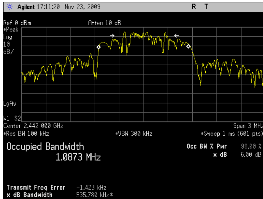
Plot 7. Occupied Band Width, Mid Channel, 6dB Bandwidth
