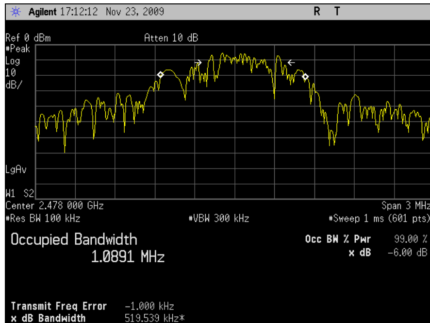
Plot 8. Occupied Band Width, High Channel, 6dB Bandwidth
