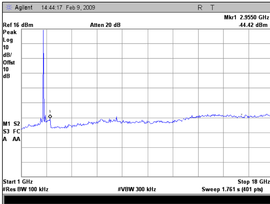
Plot 28. High Channel, Conducted Emissions, 1 GHz – 18 GHz
