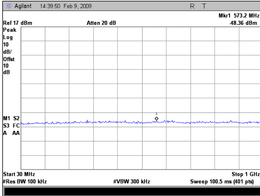
Plot 21. Low Channel, Conducted Emissions, 30 MHz – 1 GHz
