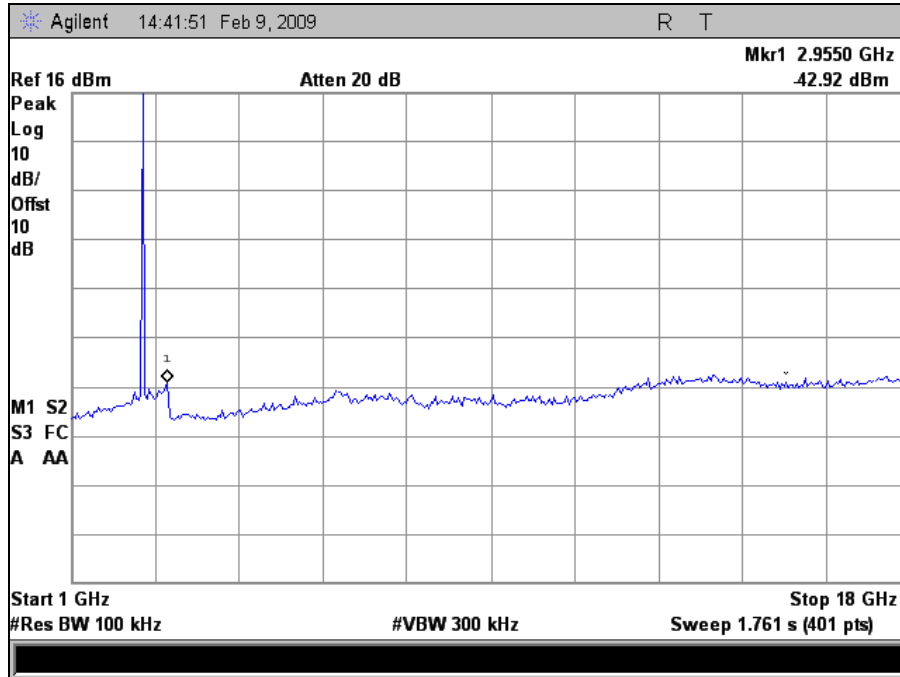
Plot 25. Mid Channel, Conducted Emissions, 1 GHz – 18 GHz
