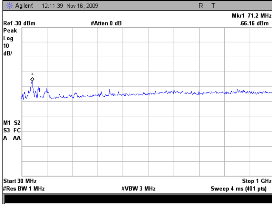
Plot 19. Receiver Spurious Emission, 30 MHz – 1 GHz
