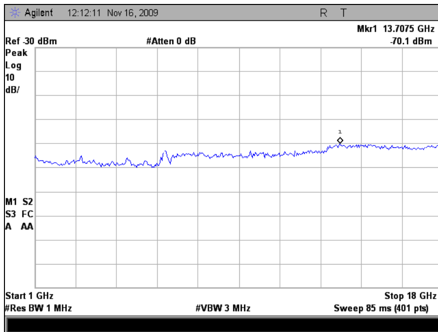
Plot 20. Receiver Spurious Emission, 1 GHz – 18 GHz
