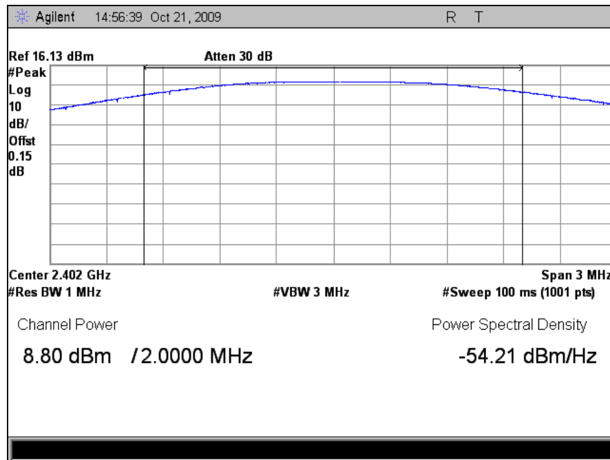
Plot 9. Peak Output Power, Low Channel
