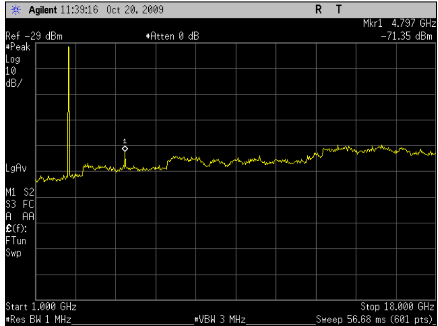
Plot 12. Radiated Spurious Emissions, Low Channel
