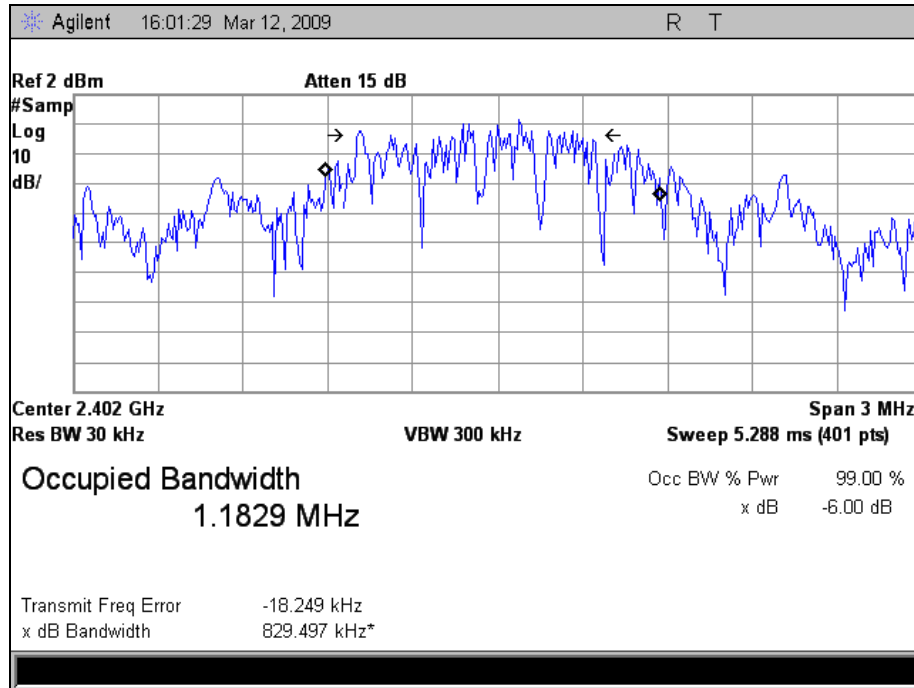
Plot 3. Occupied Band Width, Low Channel, 99 % Bandwidth
