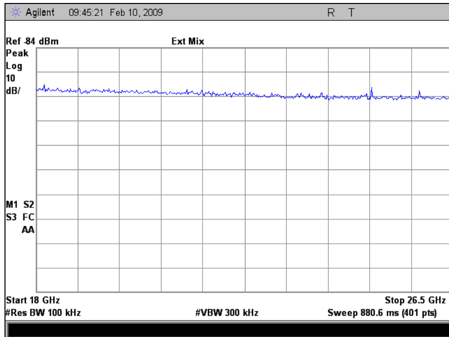
Plot 26. Mid Channel, Conducted Emissions, 18 GHz – 26 GHz
