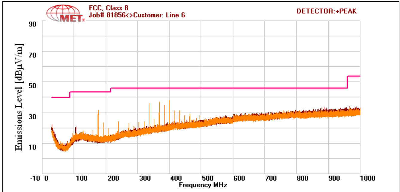
Plot 1. Radiated Emissions, Pre-Scan, FCC Limits
