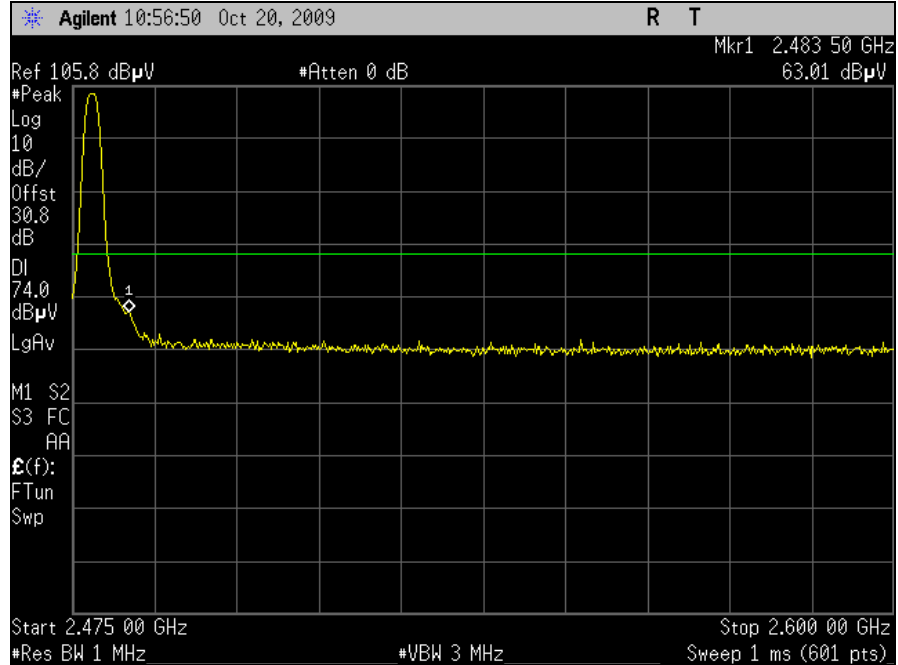
Plot 18. Upper Band Edge, Peak
