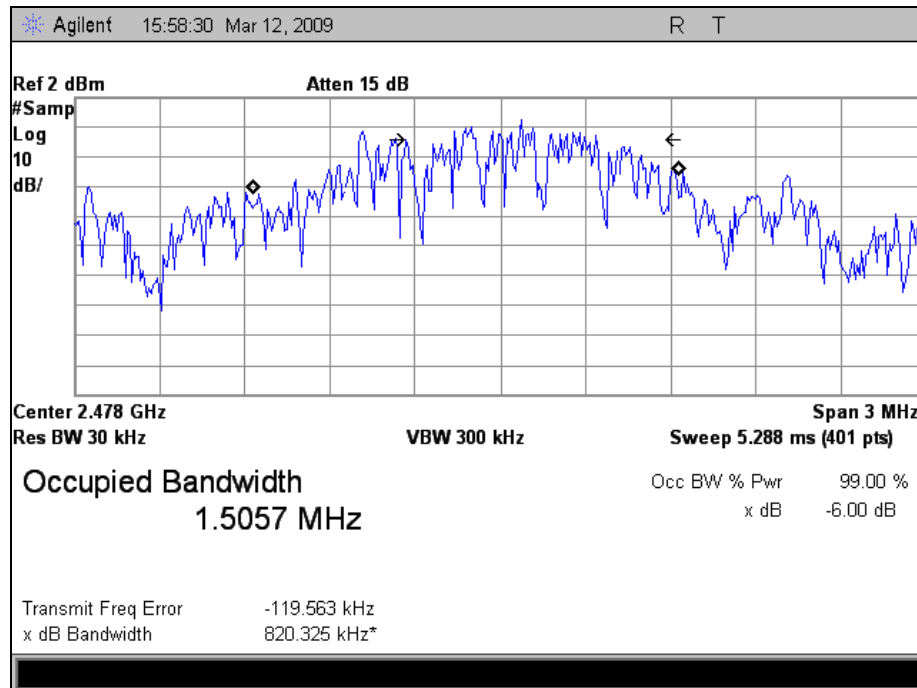
Plot 5. Occupied Band Width, High Channel, 99 % Bandwidth
