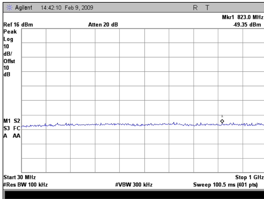
Plot 24. Mid Channel, Conducted Emissions, 30 MHz – 1 GHz
