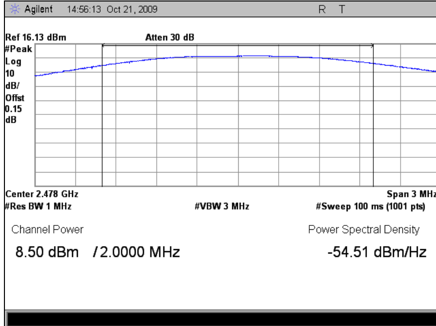
Plot 11. Peak Output Power, High Channel
