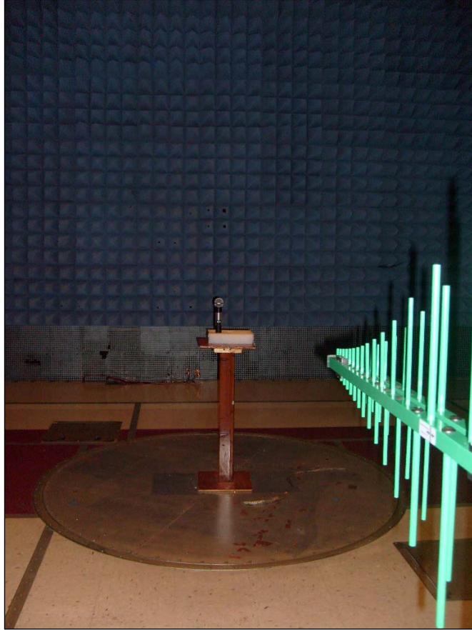
Photograph 1. Metallic Enclosure, Test Setup
