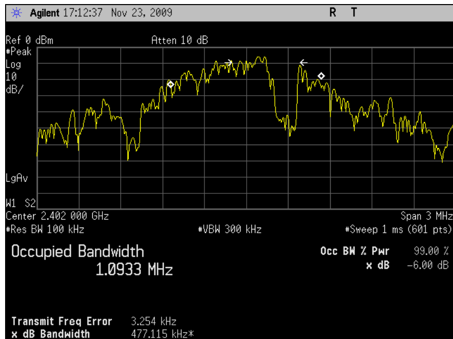
Plot 6. Occupied Band Width, Low Channel, 6dB Bandwidth
