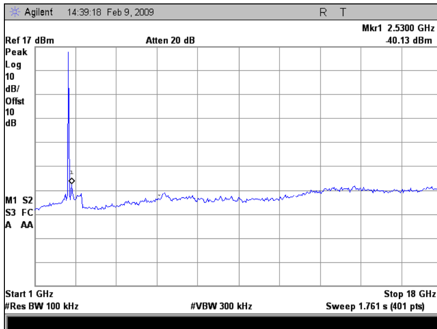
Plot 22. Low Channel, Conducted Emissions, 1 GHz – 18 GHz
