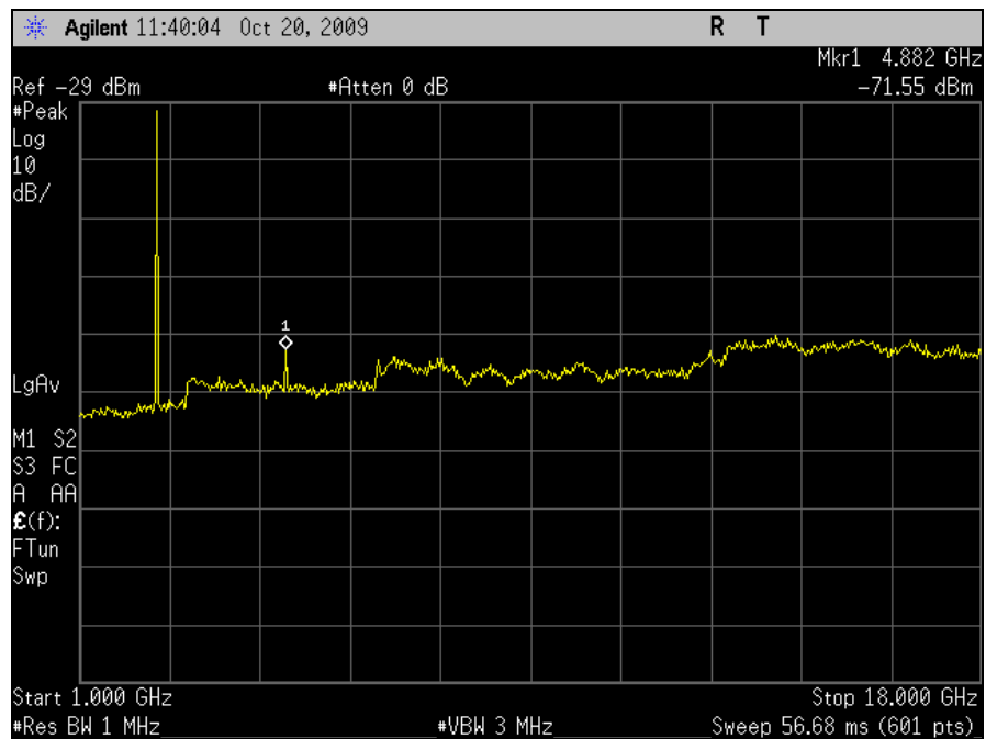
Plot 13. Radiated Spurious Emissions, Mid Channel
