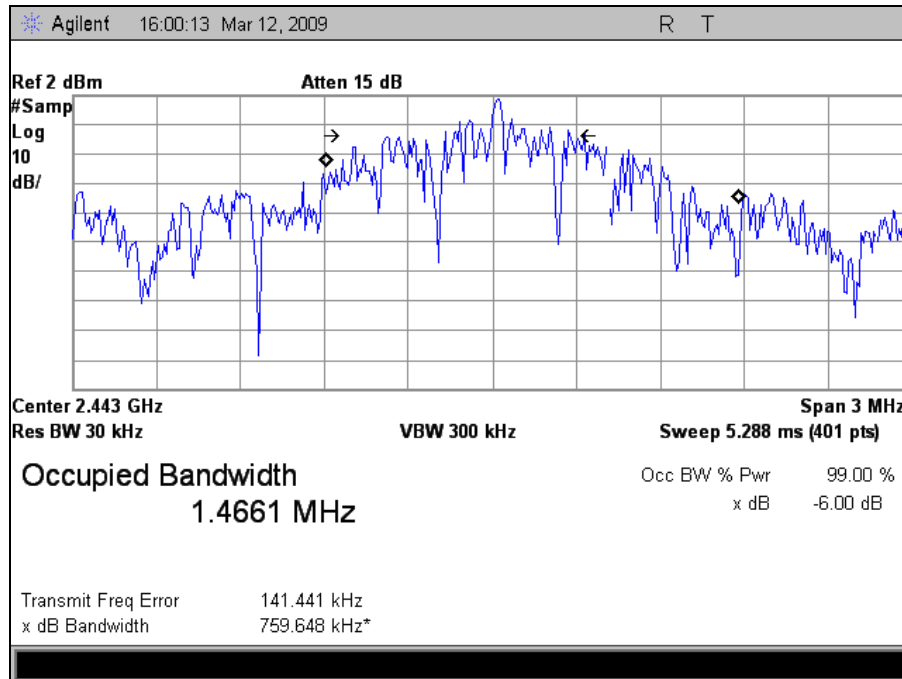
Plot 4. Occupied Band Width, Mid Channel, 99 % Bandwidth
