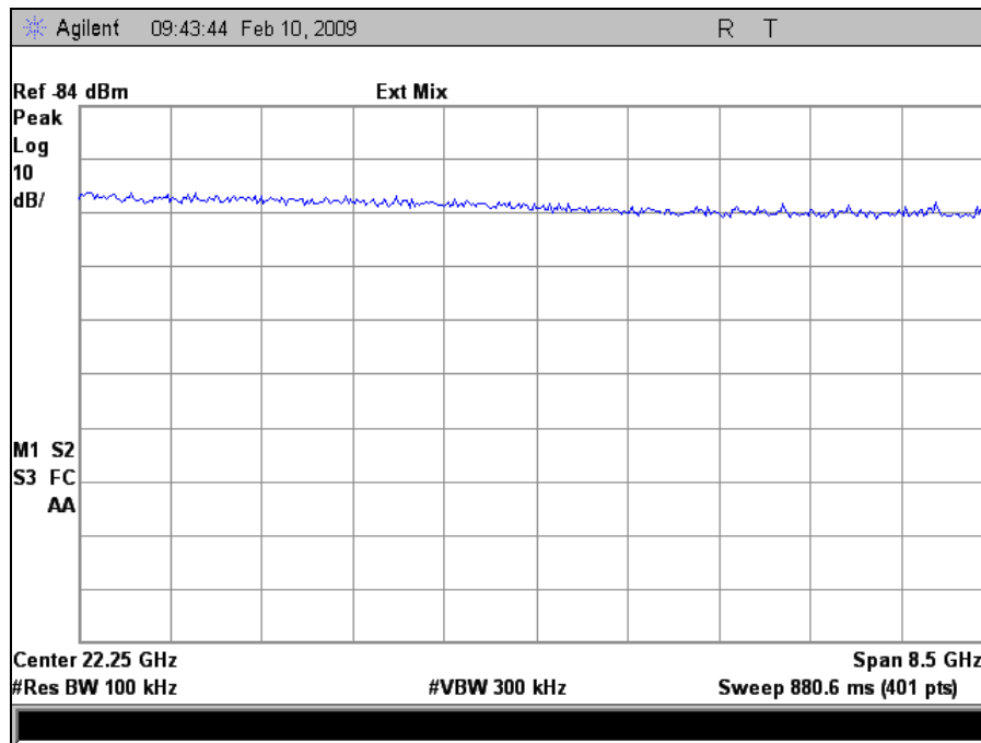
Plot 23. Low Channel, Conducted Emissions, 18 GHz – 26 GHz
