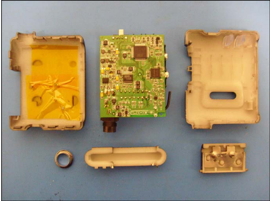
Photograph 5. Transceiver
