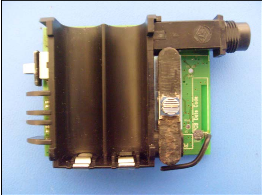
Photograph 7. Transceiver, Top
