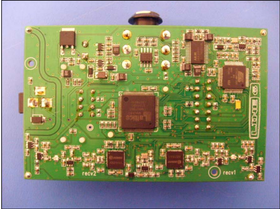
Photograph 1. Receiver Bottom
