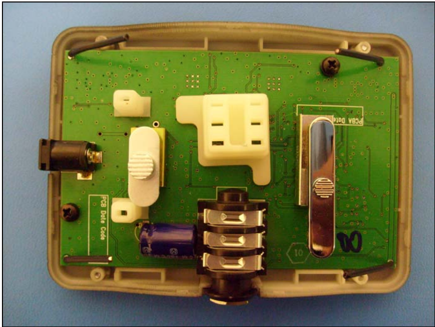
Photograph 2. Receiver Top
