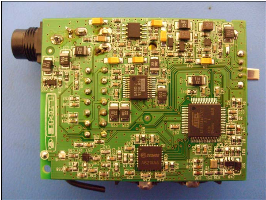
Photograph 6. Transceiver, Bottom
