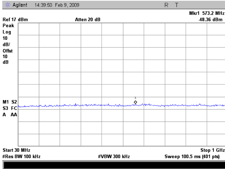
Plot 17. Low Channel Conducted Emissions 30MHz - 1GHz
