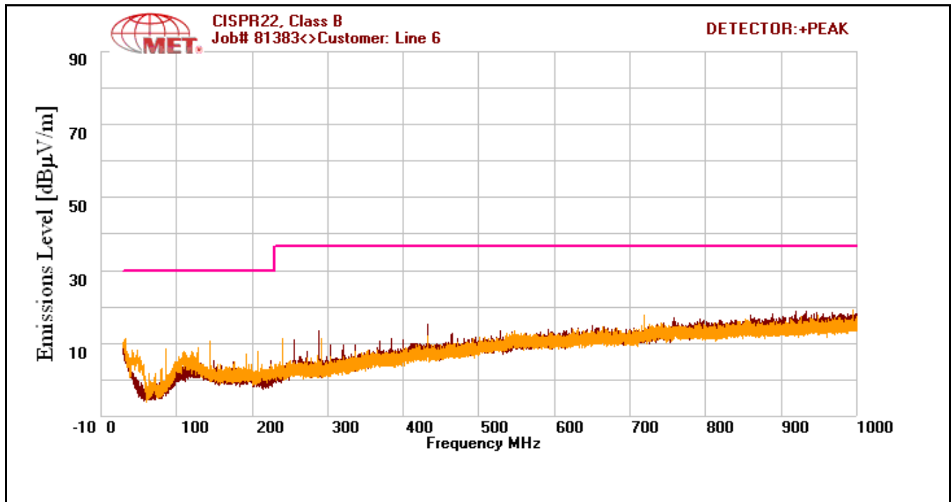
Plot 2. ICES-003 Radiated Emissions Limits Test Results, 30 MHz – 1 GHz, Class B
