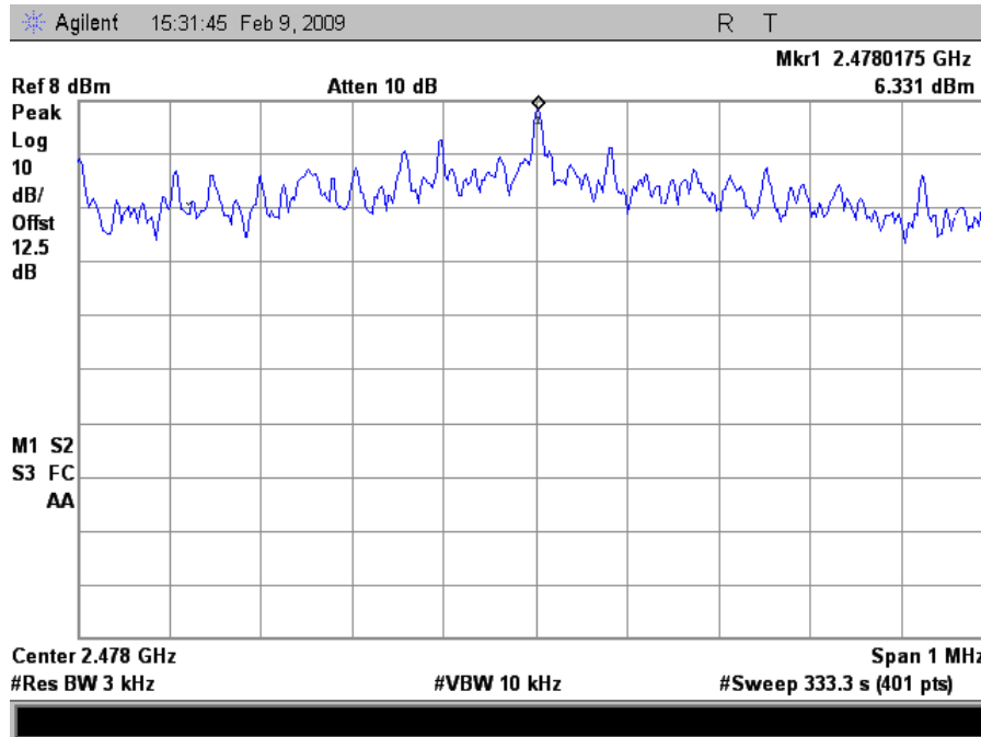
Plot 30. High Ch Peak Power Spectral Density
