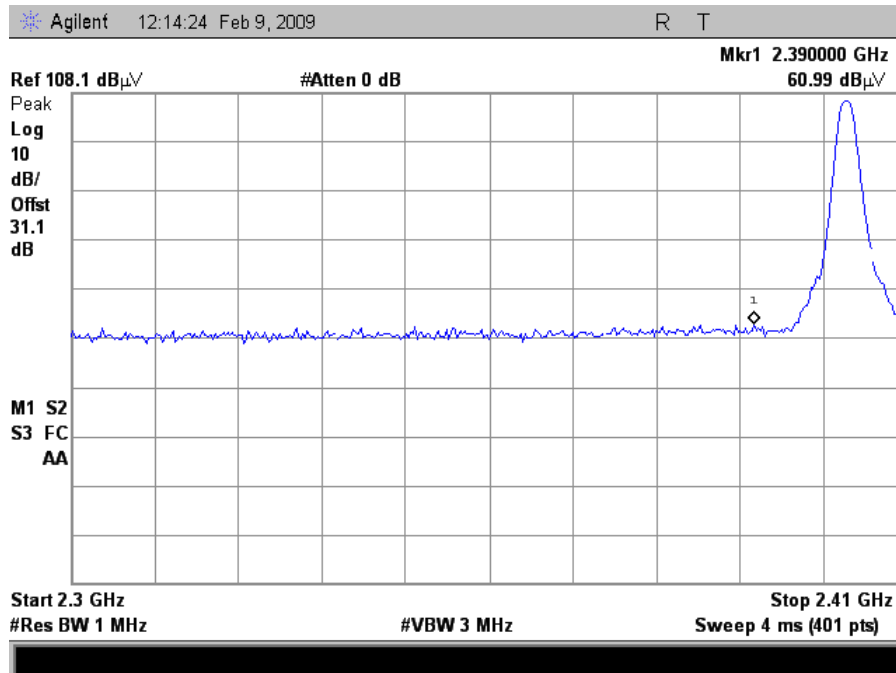
Plot 13. Low Channel Restricted Band Edge, Peak
