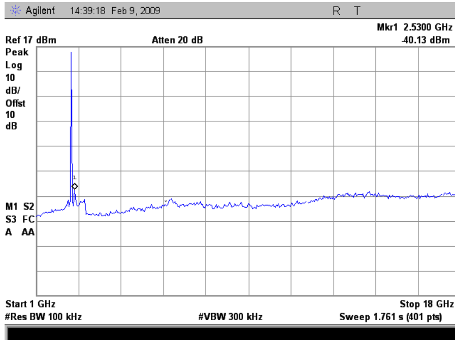
Plot 18. Low Channel Conducted Emissions 1-18GHz
