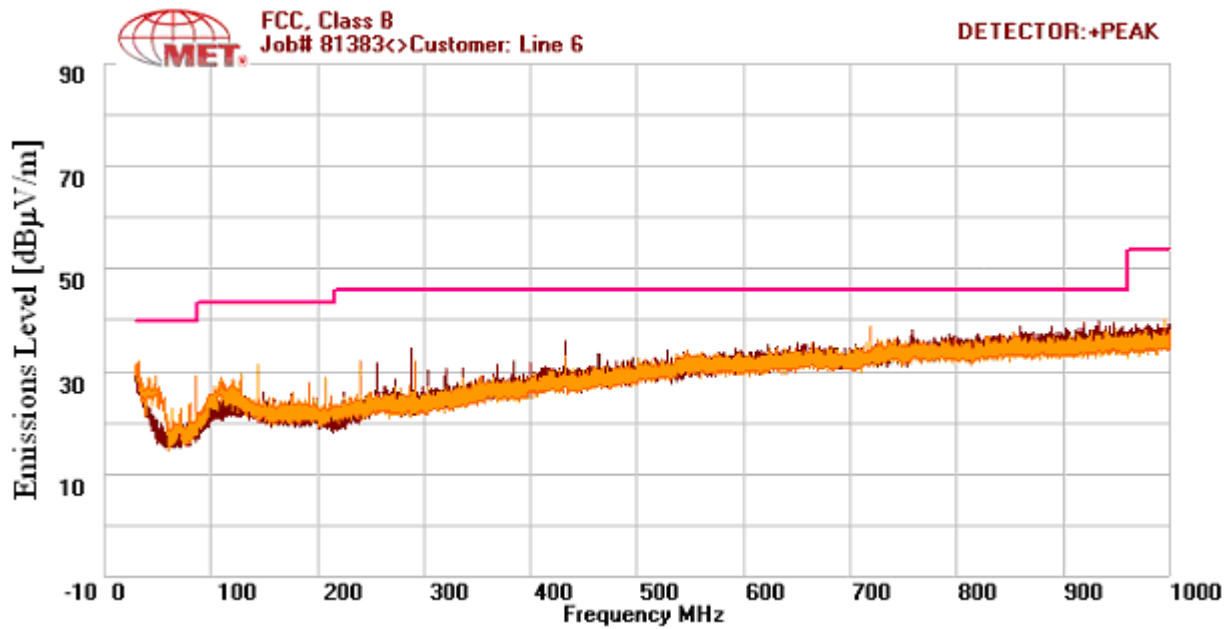
Plot 1. FCC 15B Radiated Emissions Limits Test Results, 30 MHz – 1 GHz, Class B
