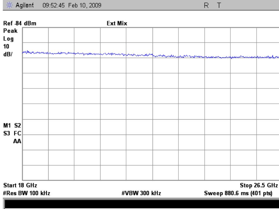
Plot 25. High Channel Conducted Emissions 18-26GHz
