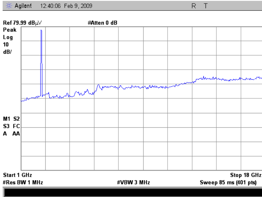
Plot 9. Low Channel Radiated Spurious, 1GHz – 18GHz
