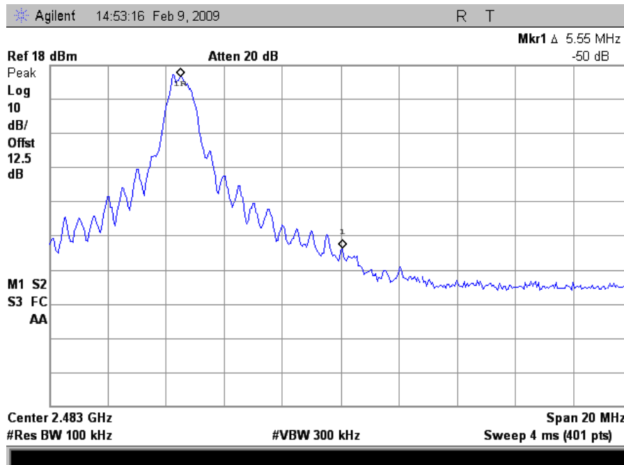
Plot 27. Conducted, Upper Band Edge
