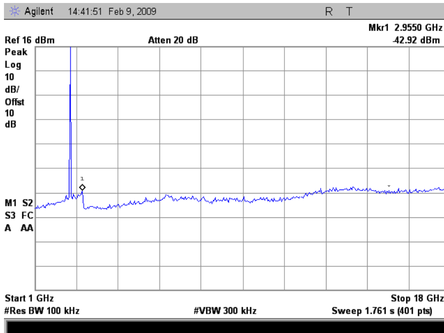
Plot 21. Mid Channel Conducted Emissions 1 - 18GHz
