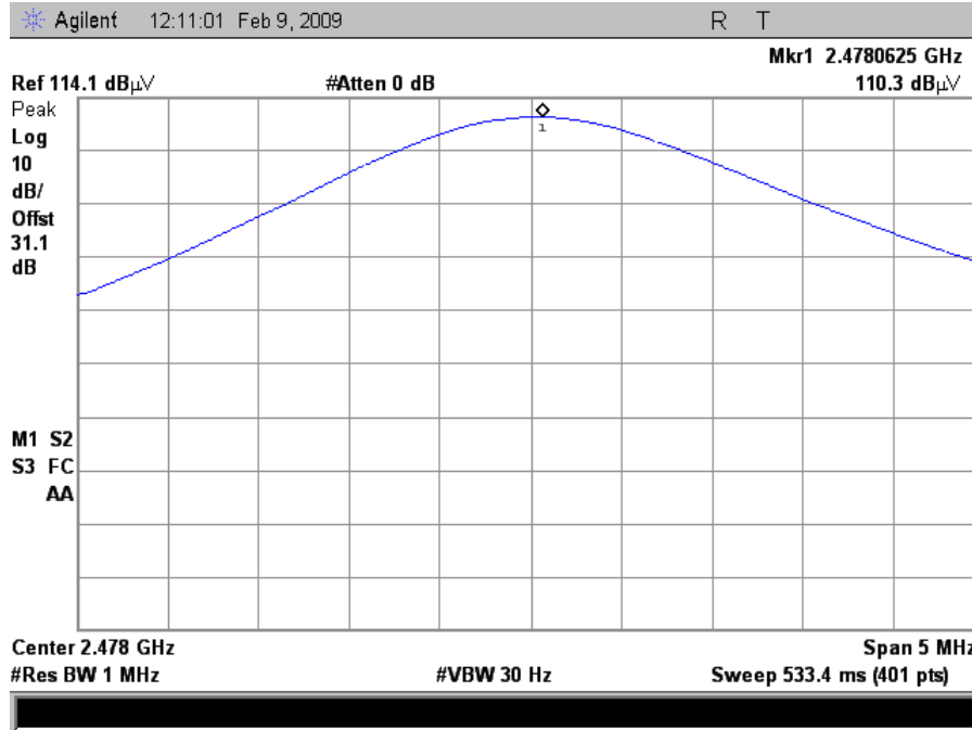
Plot 14. High Channel Restricted Band Edge, Avg
