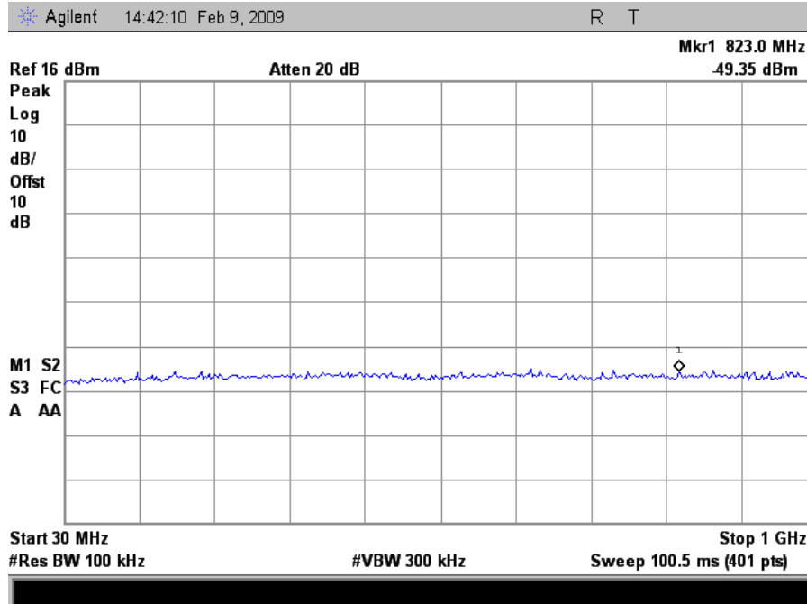
Plot 20. Mid Channel Conducted Emissions 30MHz – 1GHz
