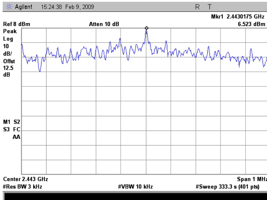
Plot 29. Mid Ch Peak Power Spectral Density
