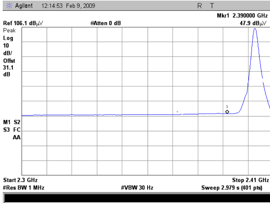
Plot 12. Low Channel Restricted Band Edge, Avg
