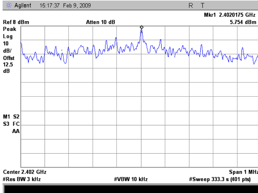
Plot 28. Low Ch Peak Power Spectral Density
