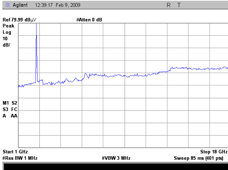
Plot 10. Mid Channel Radiated Spurious, 1GHz – 18GHz
