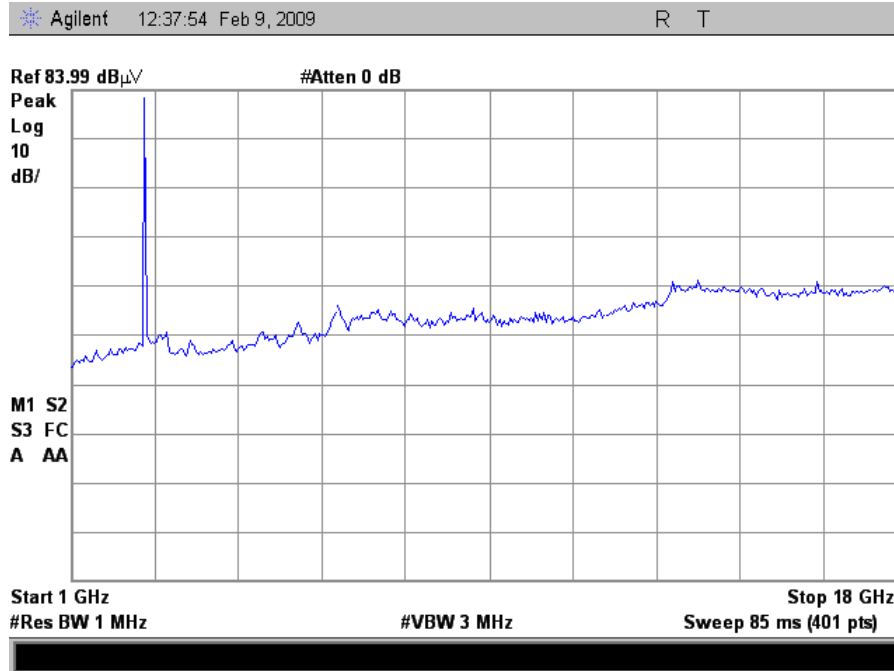
Plot 11. High Channel Radiated Spurious, 1GHz – 18GHz
