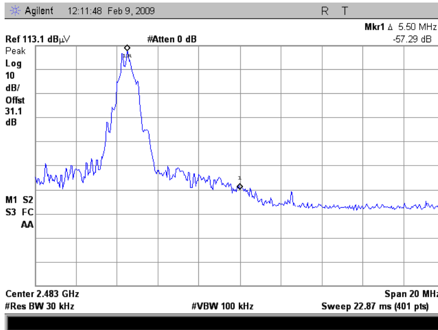
Plot 16. High Channel Restricted Band Edge, Delta
