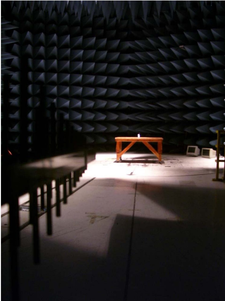
Radiated Emission Test Setup 30 MHz - 1 GHz (Transmitter)
