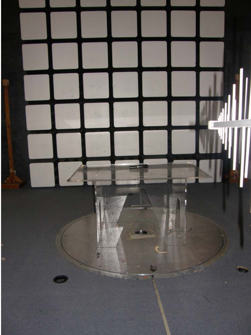
Photograph 1 Radiated Emission Test Setup 30 MHz - 1 GHz
