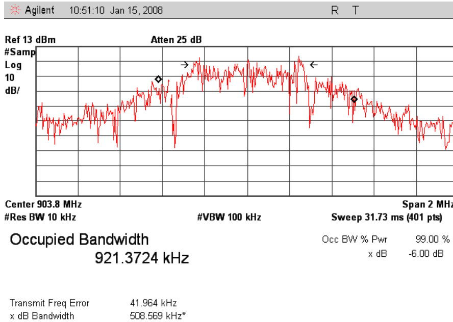
Low Ch Occupied Band Width.
