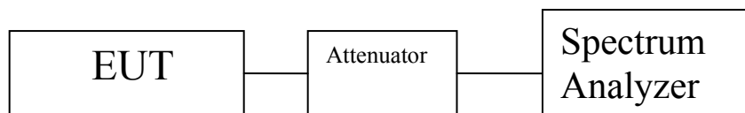
Figure 4. Block Diagram - Spurious Conducted Emissions Test Setup
