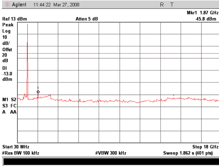
High Channel Conducted Spurious Emissions 30MHz - 18GHz
