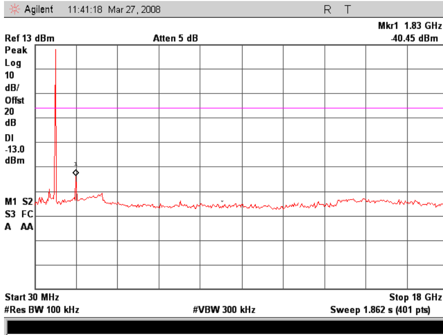
Mid Channel Conducted Spurious Emissions 30MHz - 18GHz
