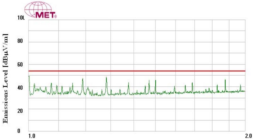
Plot 2. Radiated Emissions Limits Test Results, 1GHz – 2 GHz
