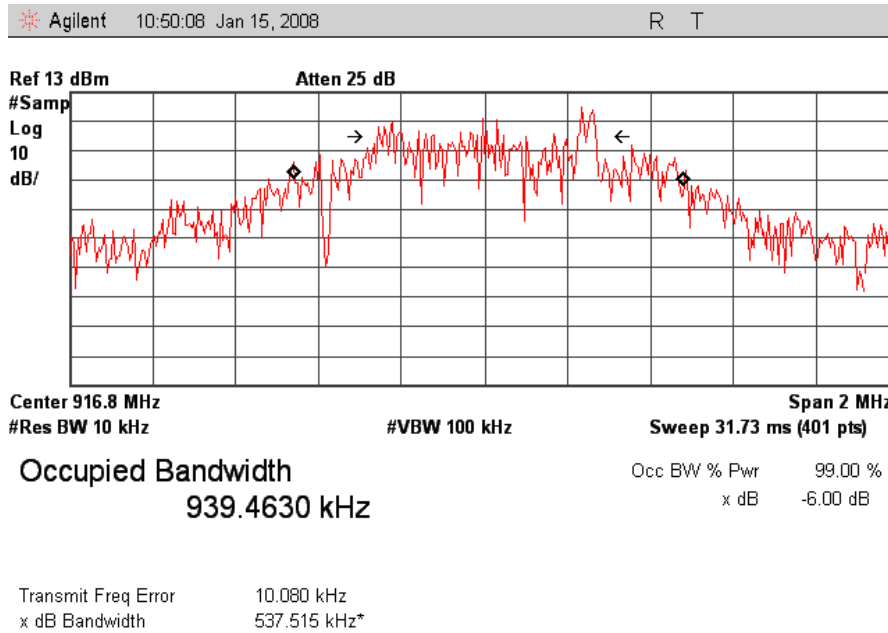
Mid Ch Occupied Band Width
