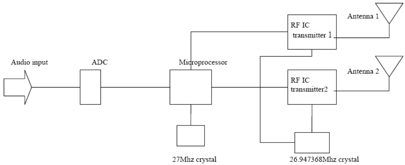
Figure 1. Block Diagram of EUT
