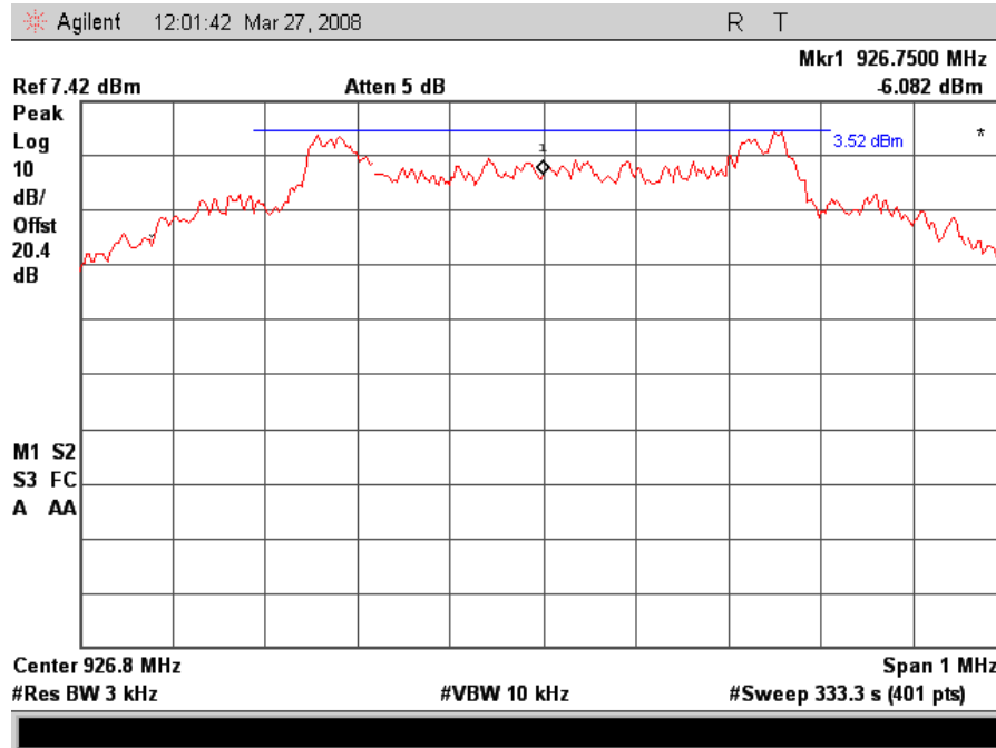
High Ch Peak Power Spectral Density
