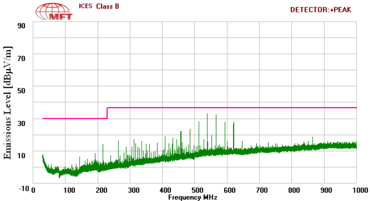
Plot 3. Radiated Emission Limits for ICES-003
