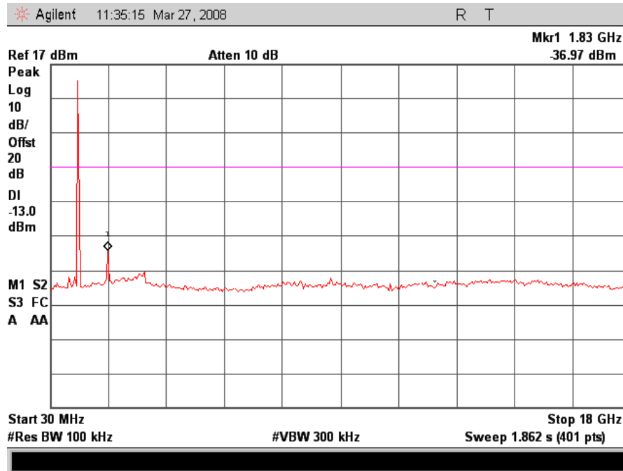
Low Channel Conducted Spurious Emissions 30MHz - 18GHz
