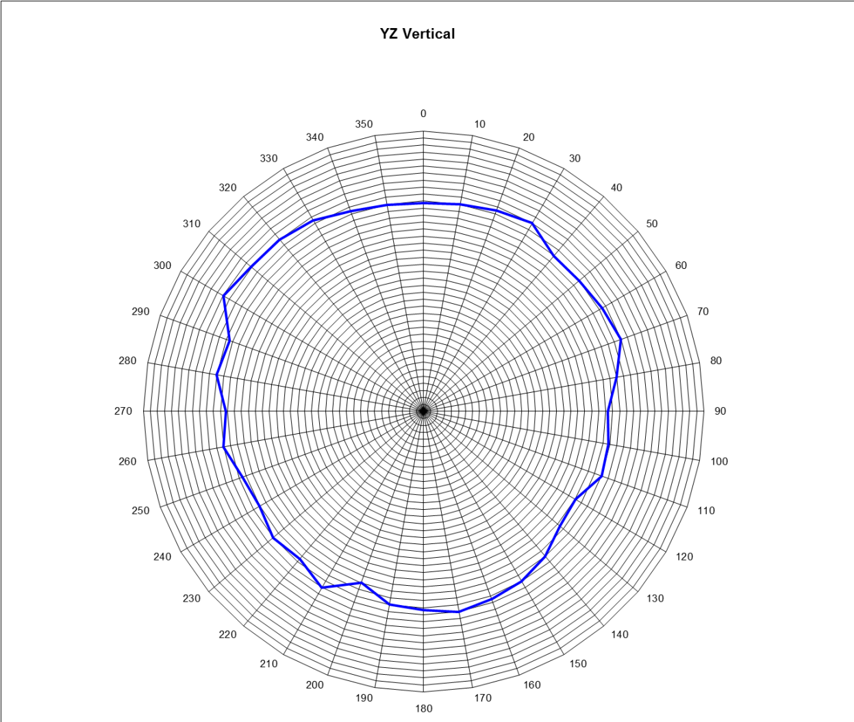
Figure 1 OdBi Ref 2400-2485MHz sweep
