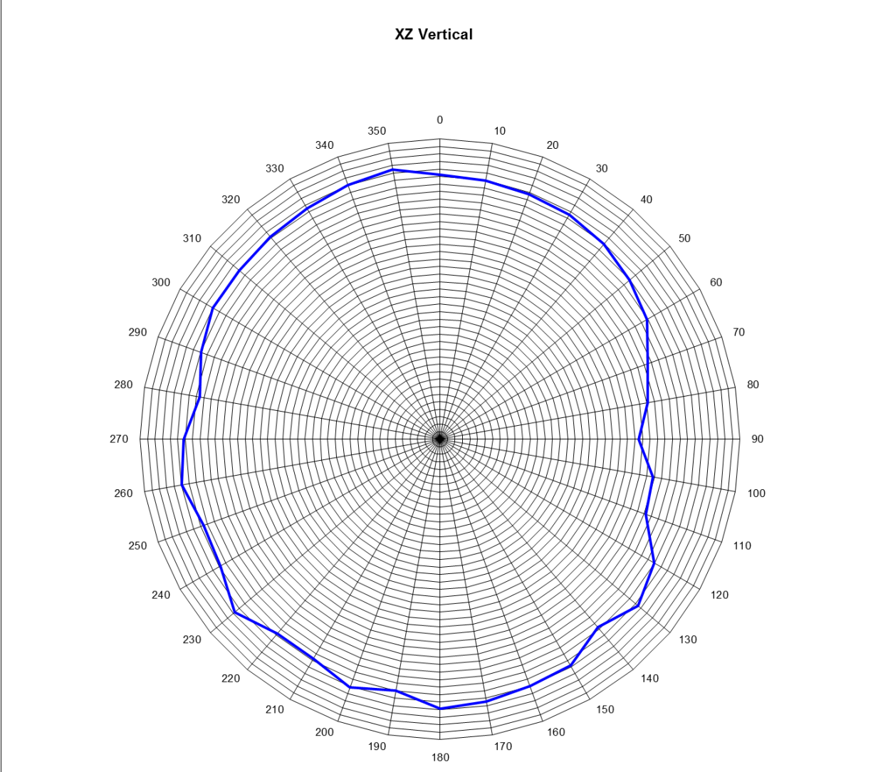
Figure 2 OdBi Ref 2400-2485MHz sweep
