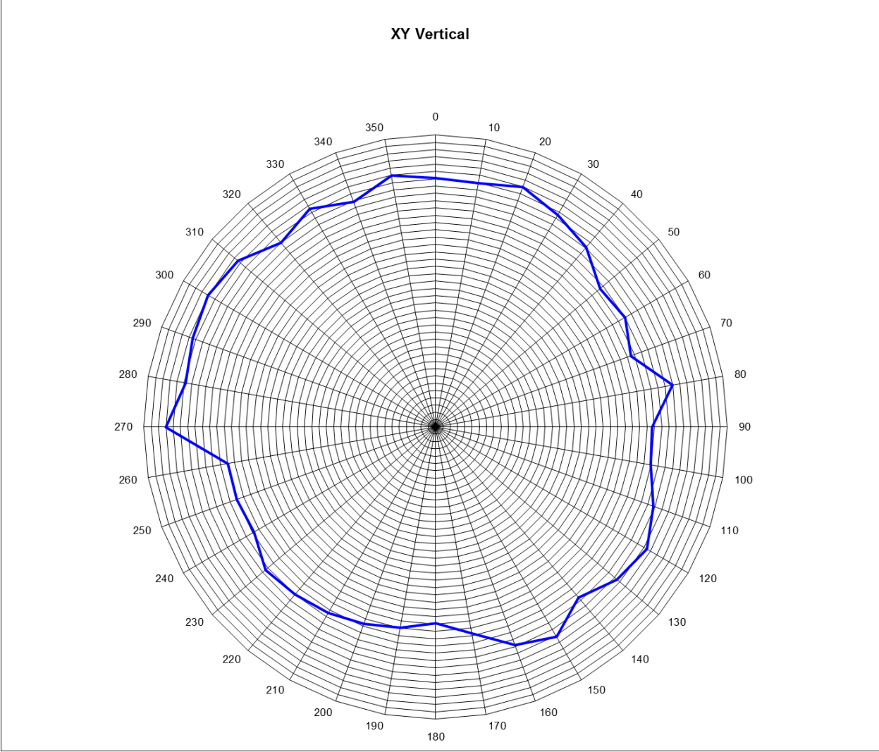
Figure 3 OdBi Ref 2400-2485MHz sweep
