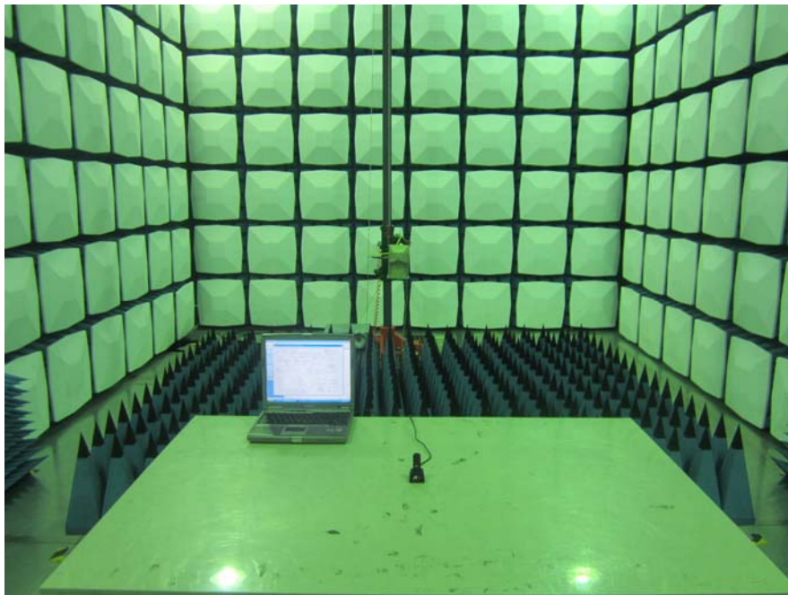
Radiated Emission -Front View (Above 1 G)
