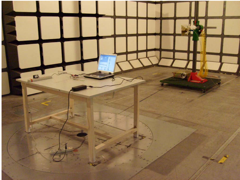
Radiated Emissions - Front View (Above 1GHz) for transmitting mode
