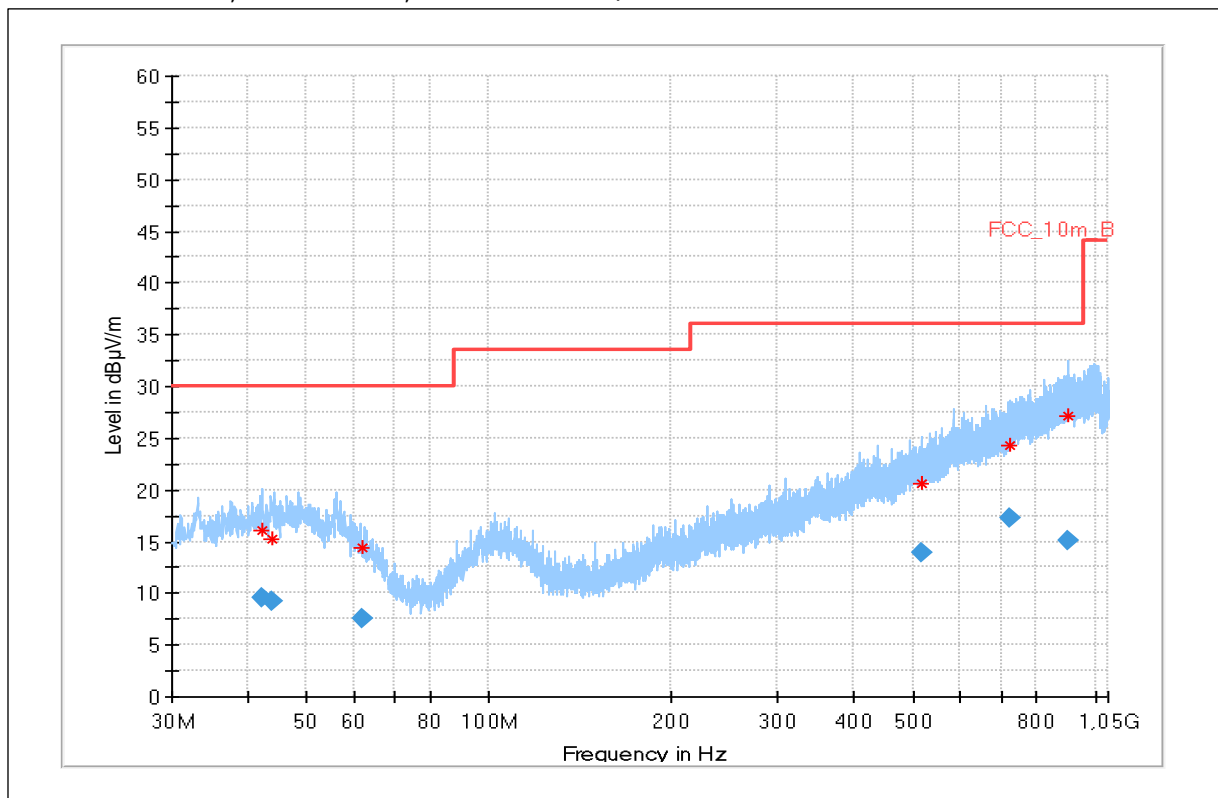
Plot 2: 30 MHz – 1 GHz, Normal Mode, antenna vertical / horizontal
