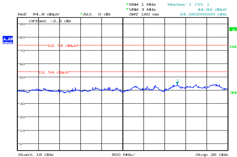
Plot 6: 18 GHz to 26 GHz, TX mode, 2480 MHz, vertical & horizontal polarization, 1 Msps
