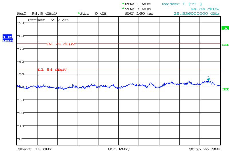
Plot 4: 18 GHz to 26 GHz, TX mode, 2440 MHz, vertical & horizontal polarization, 1 Msps
