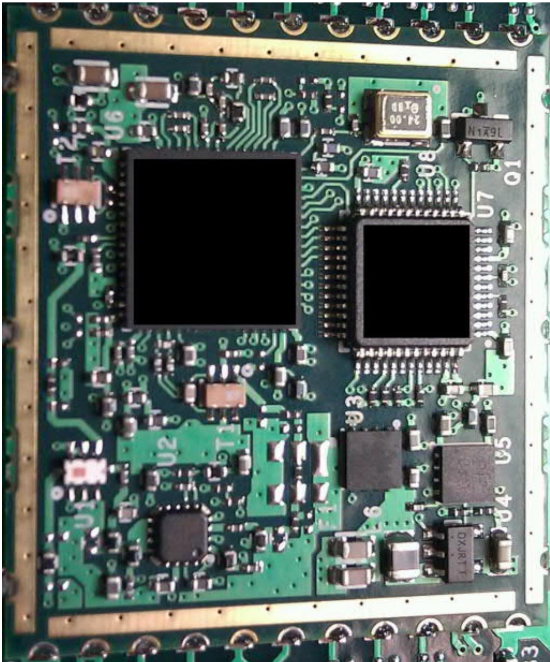
DTI901, RF PCB, bottom view, shielding removed
