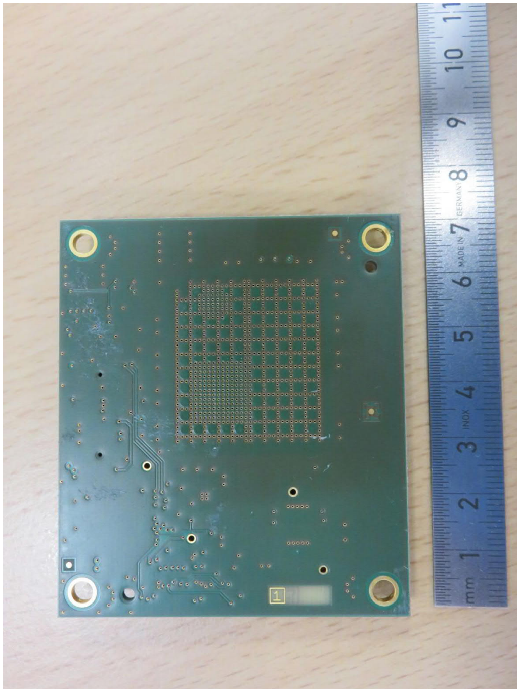
DTI901, RF PCB, top view
