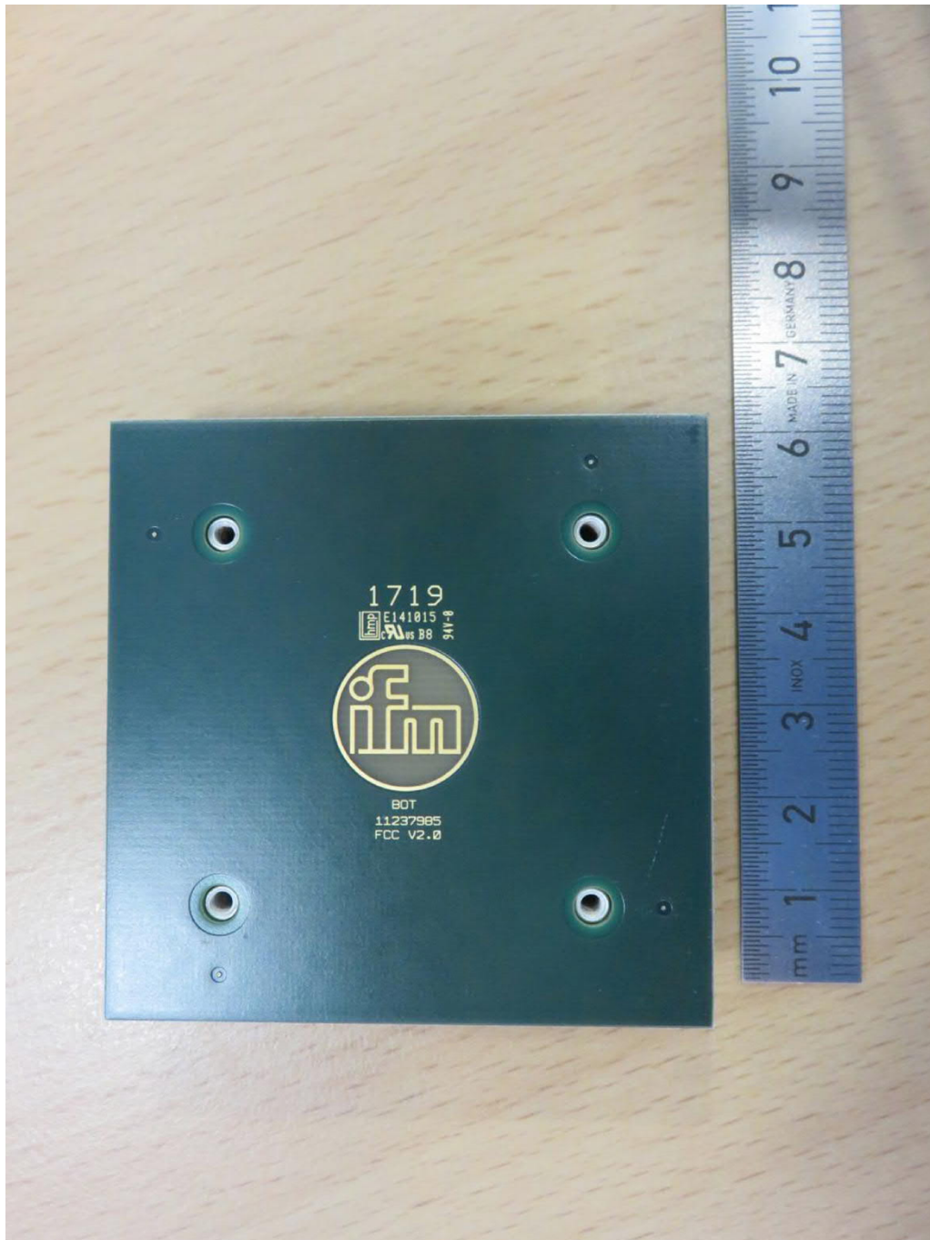
DTI901, antenna PCB 1, bottom view
