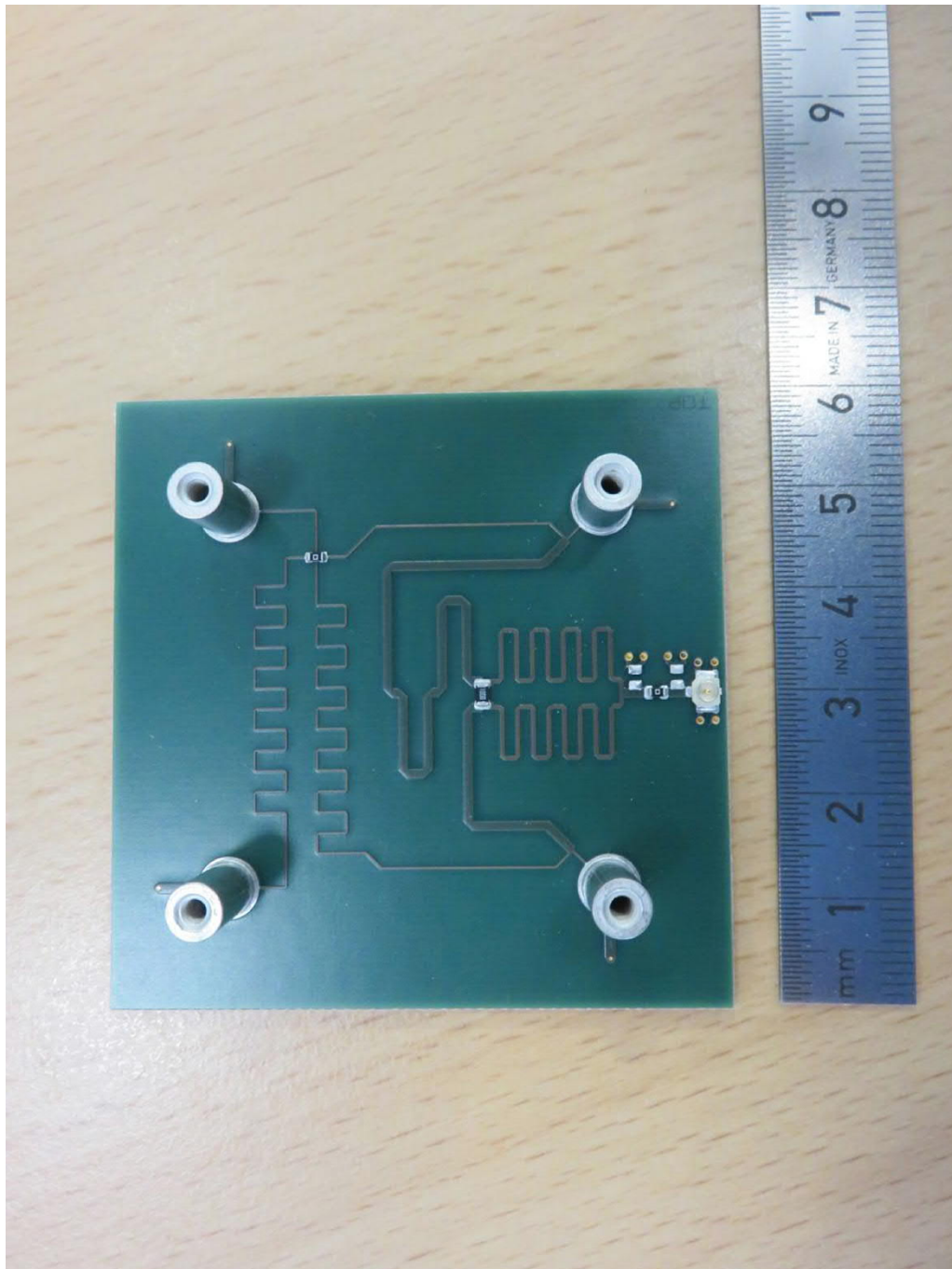
DTI901, antenna PCB 1, top view
