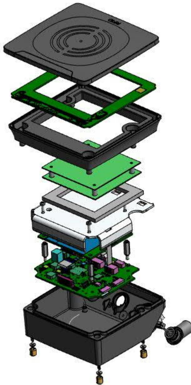
DTI901, exploded drawing
