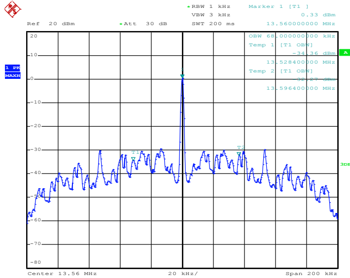
Plot 1: 99 % emission bandwidth
