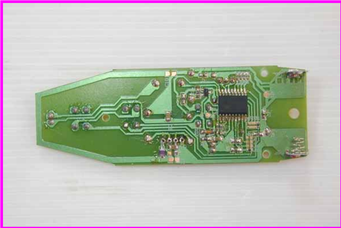
Photograph 3 Solder side of board (Transmitter)
