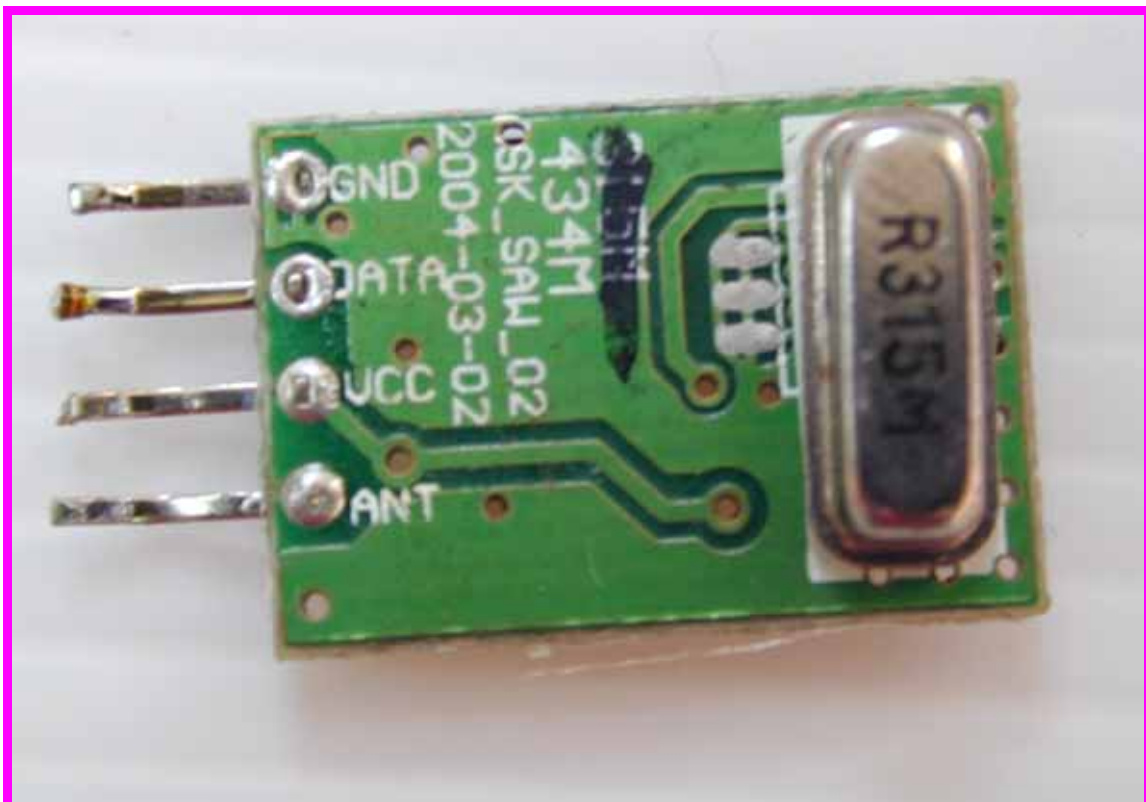
Photograph 4 Component side of board (Transmitter)
