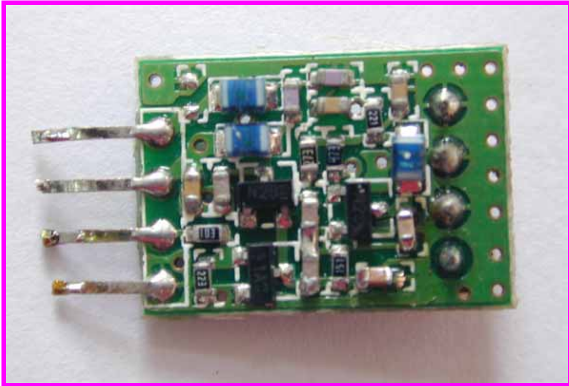
Photograph 5 Solder side of board (Transmitter)
