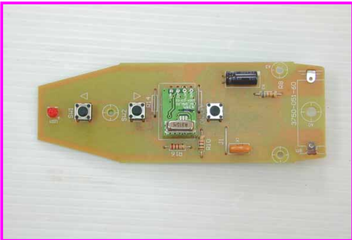
Photograph 2 Component side of board (Transmitter)
