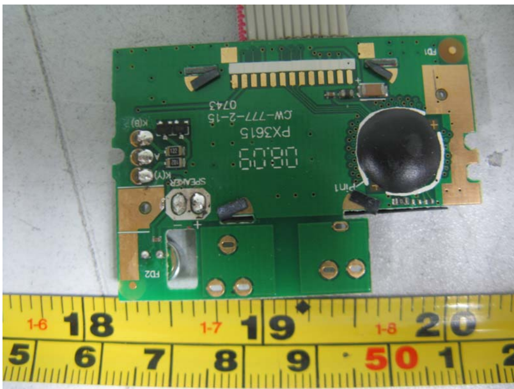
EUT – LED Board Bottom Components View
