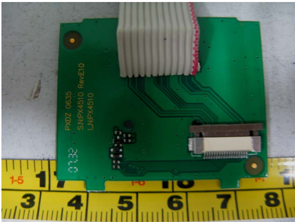
EUT – Key Board Bottom Components View
