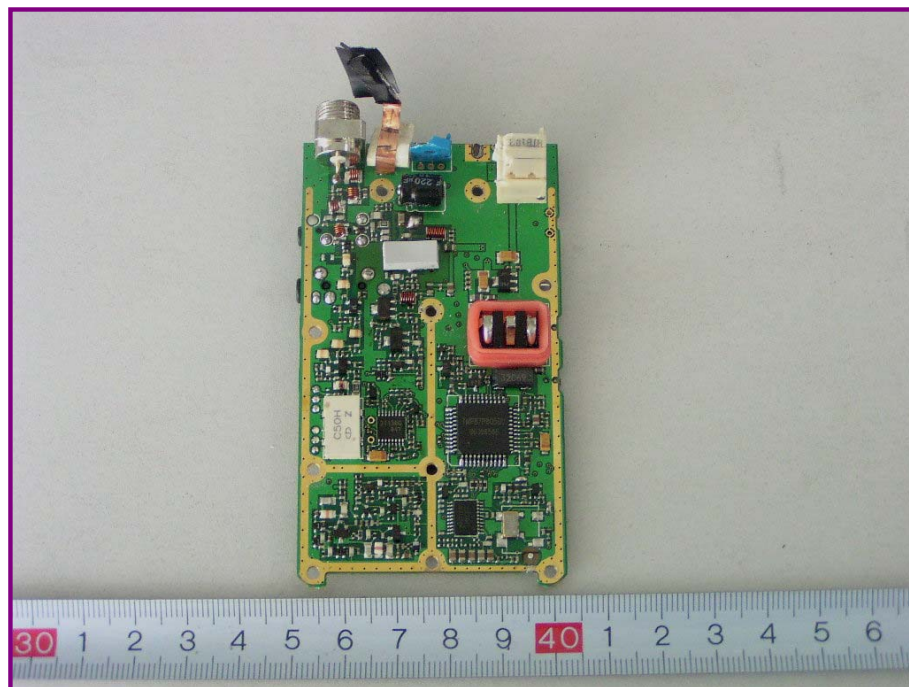
EUT- Main board PCB Top View
