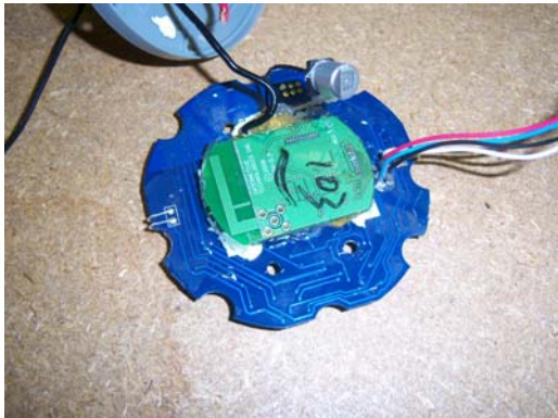
MC1 board
