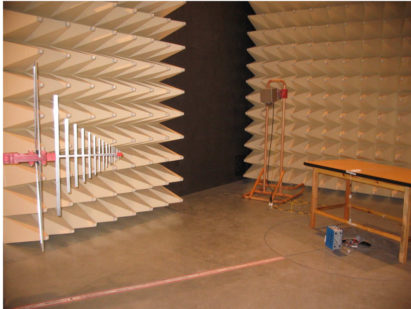
Photograph 1: Set-up for radiated emissions
